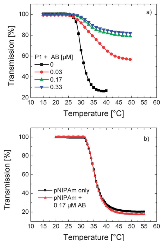
Fig. 5 Temperature-transmission profiles of (a) P1 solution in PBS ( 0.1 \text{ g L}^{-1} ) containing varying amounts of the antibody (AB) (0, 0.03, 0.17, and 0.33 \mu\text{M} ) and (b) a solution of unlabelled pNIPAm in PBS ( 0.01 \text{ g L}^{-1} ) in the presence (red triangles) and absence of the antibody ( 0.17 \mu\text{M} ) (black squares).
