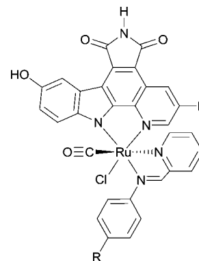
16a \text{R} = \text{H} ( \Delta -FL172) \text{IC}_{50} = 130 \text{ nM} 16b \text{R} = \text{CH}_3 ( rac -FL224) 4% inhibition at 100 nM 16c \text{R} = \text{F} ( rac -FL252) no inhibition at 100 nM
