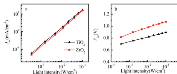
Fig. 4 The light intensity dependence of J_{\text{sc}} (a) and V_{\text{oc}} (b) in spiro-OMeTAD/ \text{CH}_3\text{NH}_3\text{PbI}_3/\text{ZrO}_2 (or \text{TiO}_2 ) solar cells.
