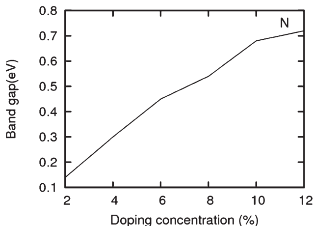
Fig. 8 Band gap in increasing order of doping concentrations (for the configuration having a maximum band gap) for N.
