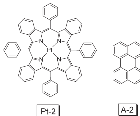
Fig. 9 Molecular structures of triplet sensitizer platinum(II) tetraphenyltetraethylporphyrin ( Pt-2 ) and the triplet acceptor A-2 . 30
