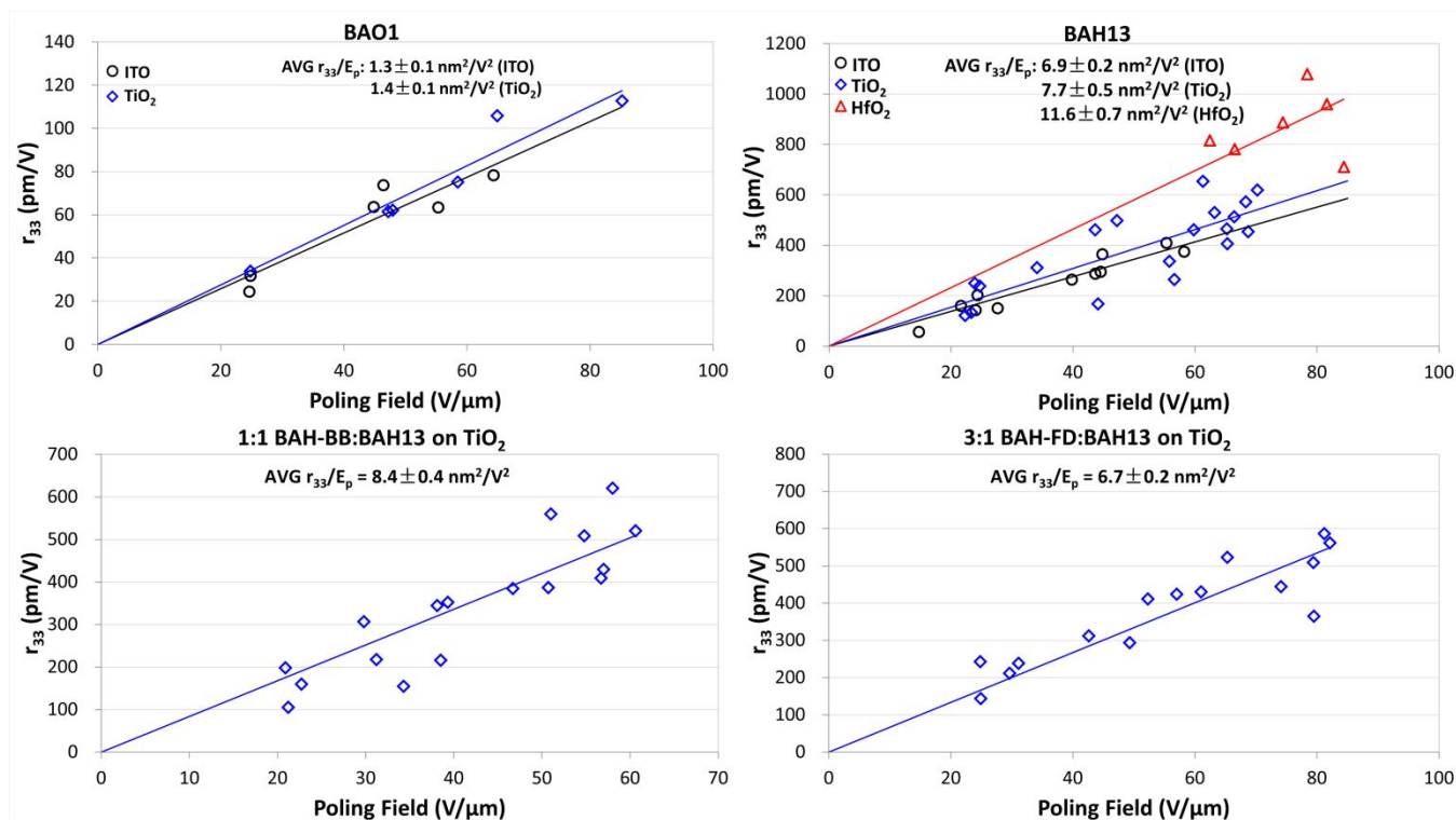
Figure 4. Poling curves for BAH chromophores (plots of r_{33} vs poling field). E_p is the average of poling fields at poling temperature and cooling down to 35°C.
