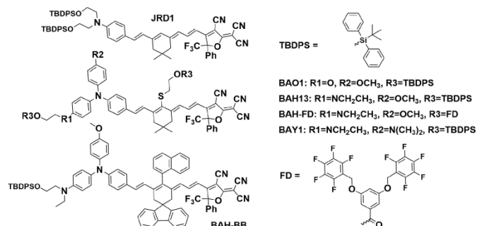
Figure 2. Chromophore structures in this study.
