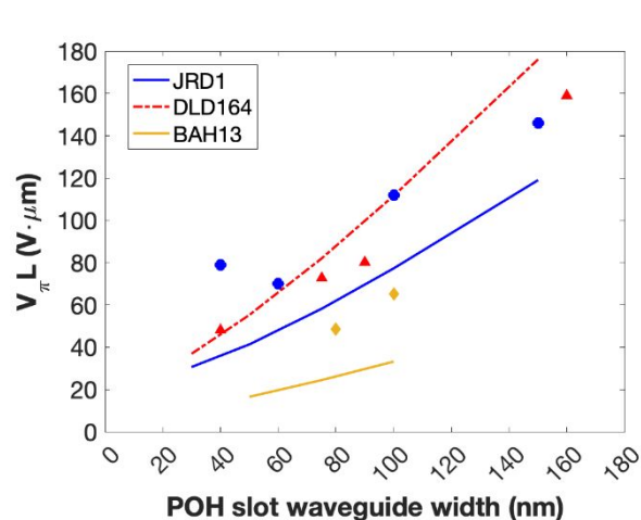
Figure 6. Comparison of measured (symbols) and computationally predicted (lines) V_{\pi}L values for JRD1, DLD164, 39,55 and BAH13 at 1550 nm in a POH MZI configuration. Measured values for JRD1 and DLD164 are from Ref. 55 ; predictions use the methodology in Ref. 72 . No CBLs were included in the waveguide calculations. Calculations are discussed in ESI†.
