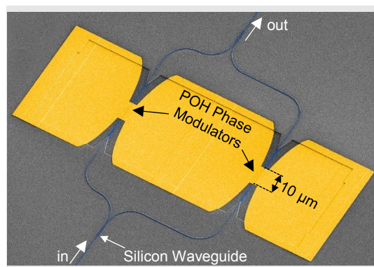
Figure 5. Colorized scanning-electron microscope picture of a POH Mach-Zehnder modulator.
