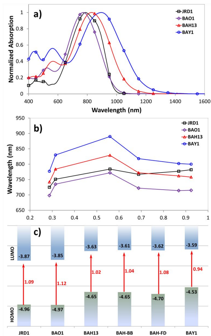
Figure 3. a) Normalized UV-vis-NIR spectra of chromophores in chloroform. b) \lambda_{\max} vs. solvent polarity on the Reichardt scale ( (\epsilon - 1)/(\epsilon + 2) ) spanning a range of dielectric constants from 1,4-dioxane ( \epsilon = 2.2 ) to acetonitrile ( \epsilon = 37.5 ). c) HOMO from cyclic voltammetry (CV) and LUMO energy levels and thin film optical energy gaps, in eV; LUMO = HOMO (CV) + Band gap (optical).
