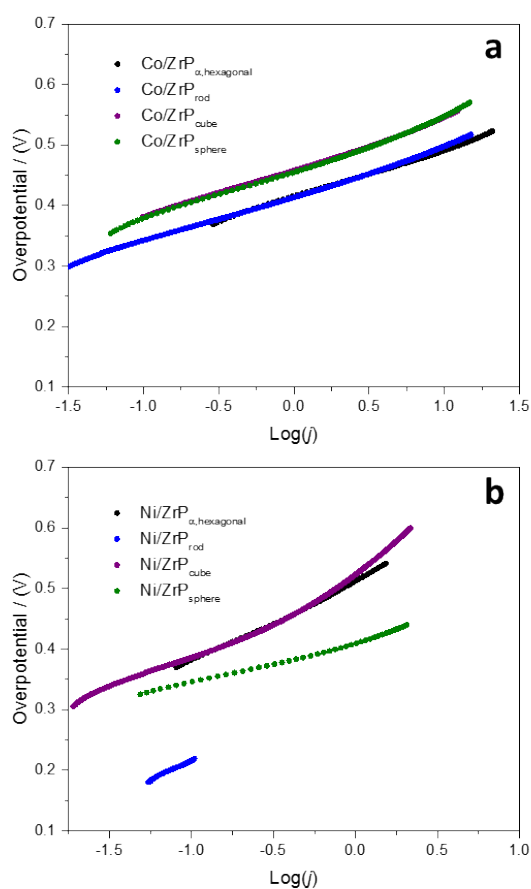
Figure 5. Tafel plots of (a) Co/ZrP catalysts and (b) Ni/ZrP catalysts.
