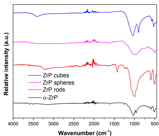
Figure 2. FTIR spectra of \alpha -ZrP, rod-like ZrP, spherical ZrP, and cube-like ZrP ( \tau' -ZrP).
