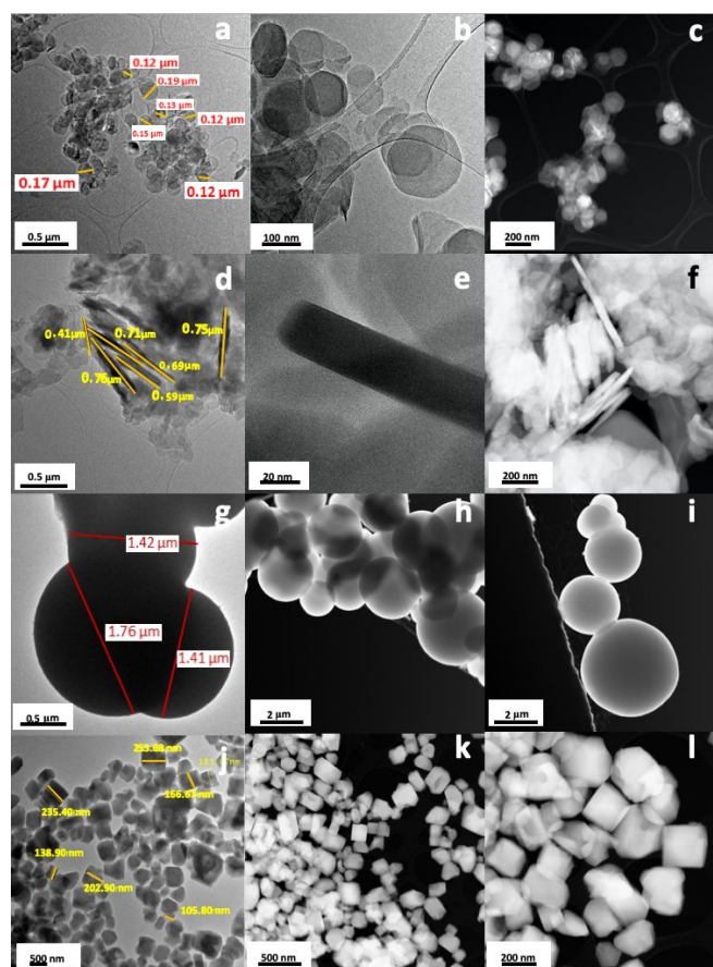
Figure 3. (a-c) TEM/STEM micrographs of \alpha -ZrP. Scale bars: 0.5 \mu\text{m} , 100 nm, and 200 nm, respectively. (d-f) TEM/STEM micrographs of rod-like ZrP. Scale bars: 0.5 \mu\text{m} , 20 nm, and 200 nm, respectively. (g-i) TEM/STEM micrographs of spherical ZrP. Scale bars: 0.5 \mu\text{m} , 2 \mu\text{m} , and 2 \mu\text{m} , respectively. (j-l) TEM/STEM
