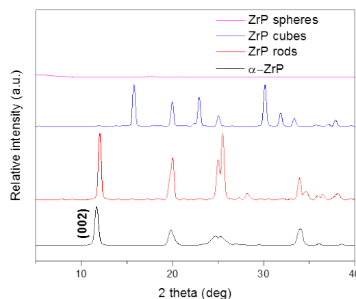
Figure 1. XRPD patterns of \alpha -ZrP, rod-like ZrP, cube-like ZrP ( \tau' -ZrP), and spherical ZrP.
