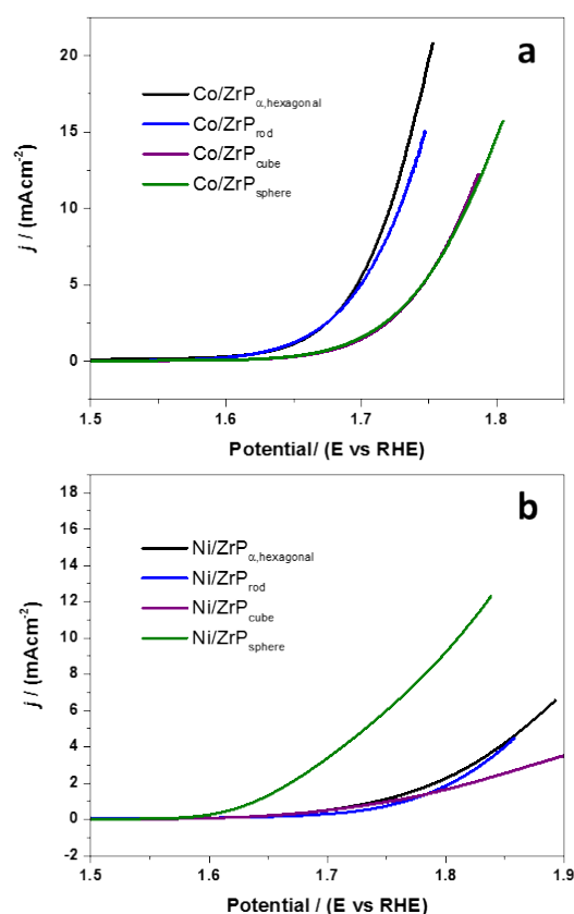
Figure 4. Linear sweep voltammograms of (a) Co/ZrP catalysts and (b) Ni/ZrP catalysts.
