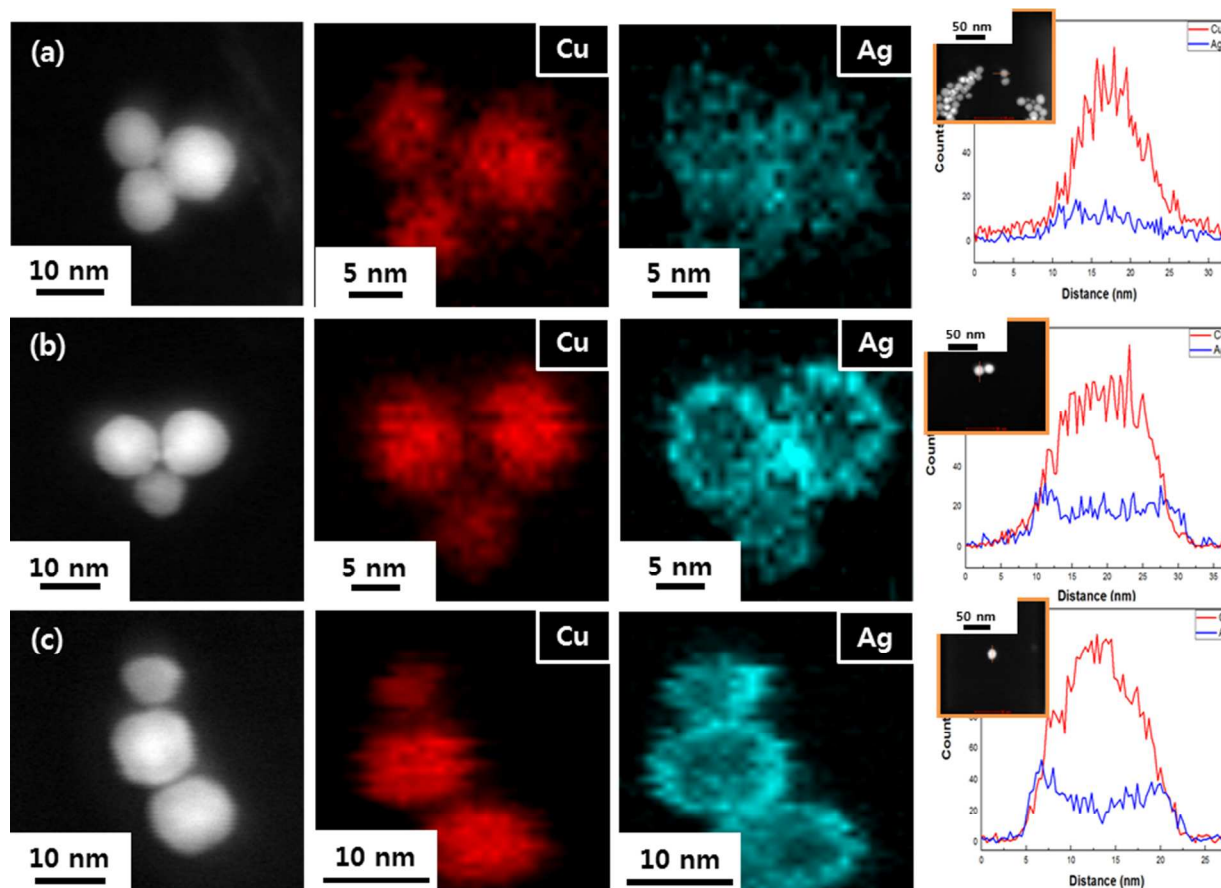
Fig. 7 Elemental mapping and line profile images of Cu@Ag NPs synthesized with different reaction temperatures for 2 h: (a) 80, (b) 130, and (c) 150 °C.
