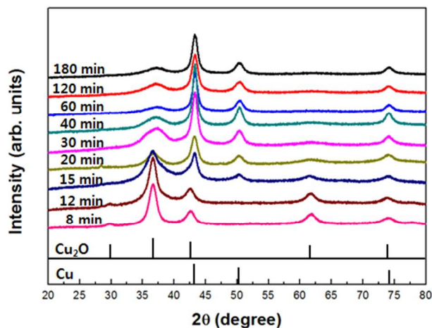
Fig. 3 XRD patterns of NPs with increasing reaction time.
