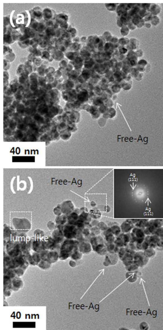
Fig. 11 TEM images of Cu@AgNPs immersed at (a) 80 °C and (b) 150 °C after annealing at 200 °C for 15 min.
