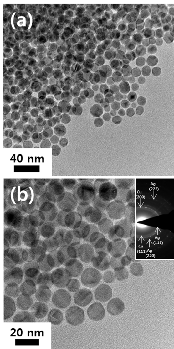
Fig. 5 TEM images of Cu@Ag core-shell NPs immersed at 80 °C for 2 h: (a) low-magnification and (b) high-magnification images with SAED pattern (inset).
