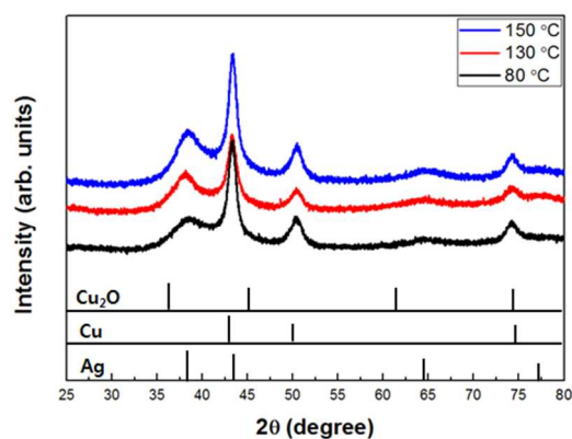
Fig. 8 XRD patterns of Cu@Ag NPs coated for 2 h at 80, 130, and 150 °C.
