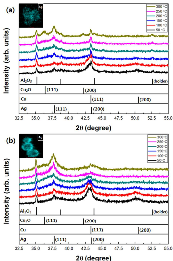
Fig. 10 High-temperature XRD patterns of Cu@Ag NPs coated at (a) 80 °C and (b) 150 °C with elemental mapping images of the Ag shell (inset).
