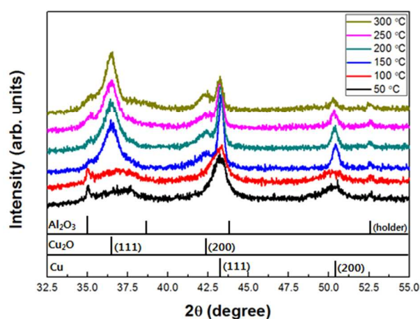
Fig. 9 High-temperature XRD patterns of Cu NPs synthesized for 3 h at 240 °C.
