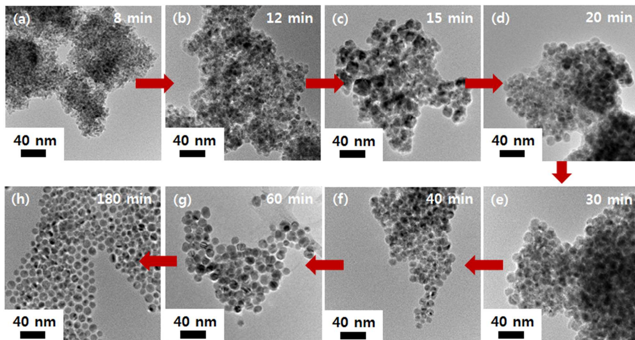
Fig. 2 TEM images of NPs as a function of reaction time in solvothermal synthesis at 240 °C.
