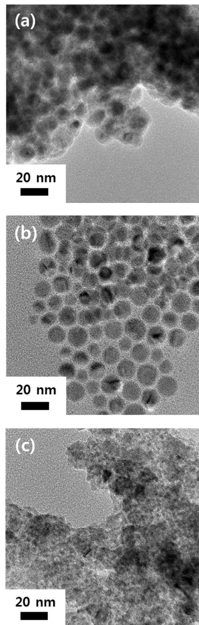
Fig. 1 TEM images of Cu NPs synthesized using a solvothermal method for 3 h at different reaction temperatures: (a) 230, (b) 240, and (c) 250 °C.
