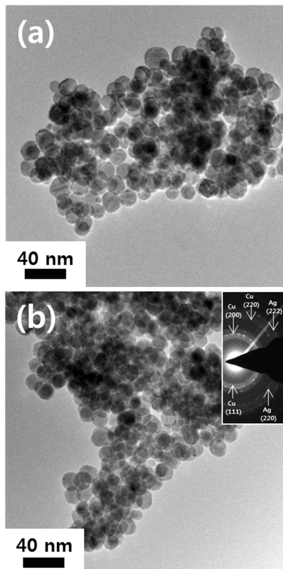
Fig. 6 TEM images of Cu@Ag core-shell NPs immersed for 2 h at (a) 130 °C and (b) 150 °C.
