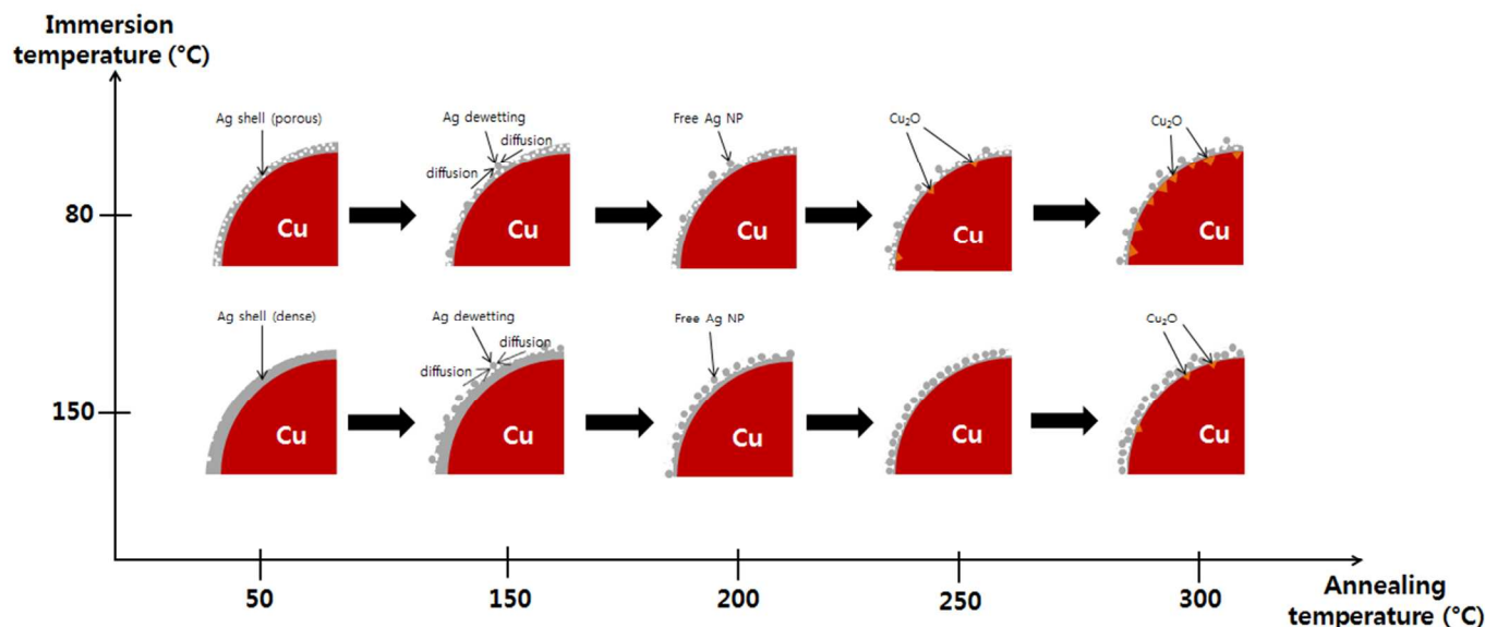
Fig. 12 Schematic images of the Ag dewetting mechanism in ultrafine Cu@Ag NPs immersed at 80 and 150 °C during annealing.
