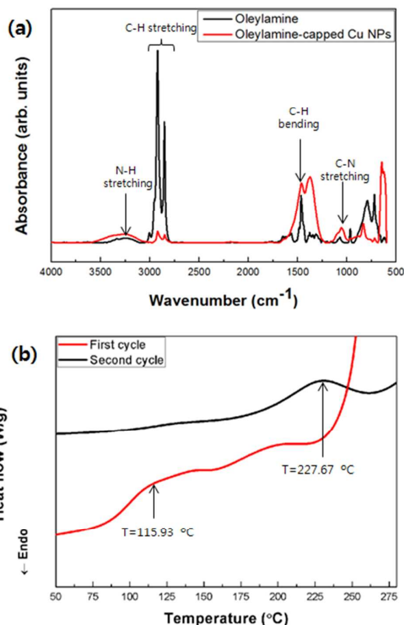
Fig. 4 (a) FT-IR spectra of Cu NPs synthesized using a solvothermal method with a pure oleylamine, and (b) DSC results of Cu NPs synthesized using a solvothermal method.
