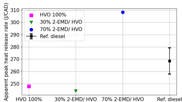
Fig. 5 Apparent peak heat release rate for 30% and 70% (v/v) blends of 2-EMD with HVO, neat HVO and reference diesel at constant IMEP and SOC.
