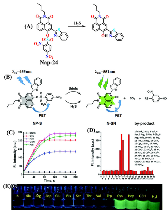
Fig. 17 (A) Structure of Nap-24 and its product formed after reaction with H 2 S. (B) The proposed sensing mechanism for the detection of H 2 S. (C) Time (0 to 200 s) vs. fluorescence intensity (I 551 ) curves of probe Nap-24 in the presence of various thiols and H 2 S in aqueous solution. (D) The fluorescence intensities (I 551 ) of Nap-24 mixed with various interferents in aqueous solution. (E) The ultraviolet light image of Nap-24 with the detection target and interfering amino acids. Reproduced with permission from ref. 75. Copyright 2019, Royal Society of Chemistry.
