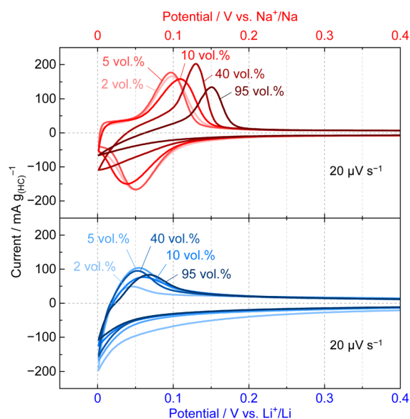
Fig. 3 Cyclic voltammograms of (top) Na and (bottom) Li cells using various diluted electrodes with a scan rate of 20 \mu\text{V s}^{-1} .
