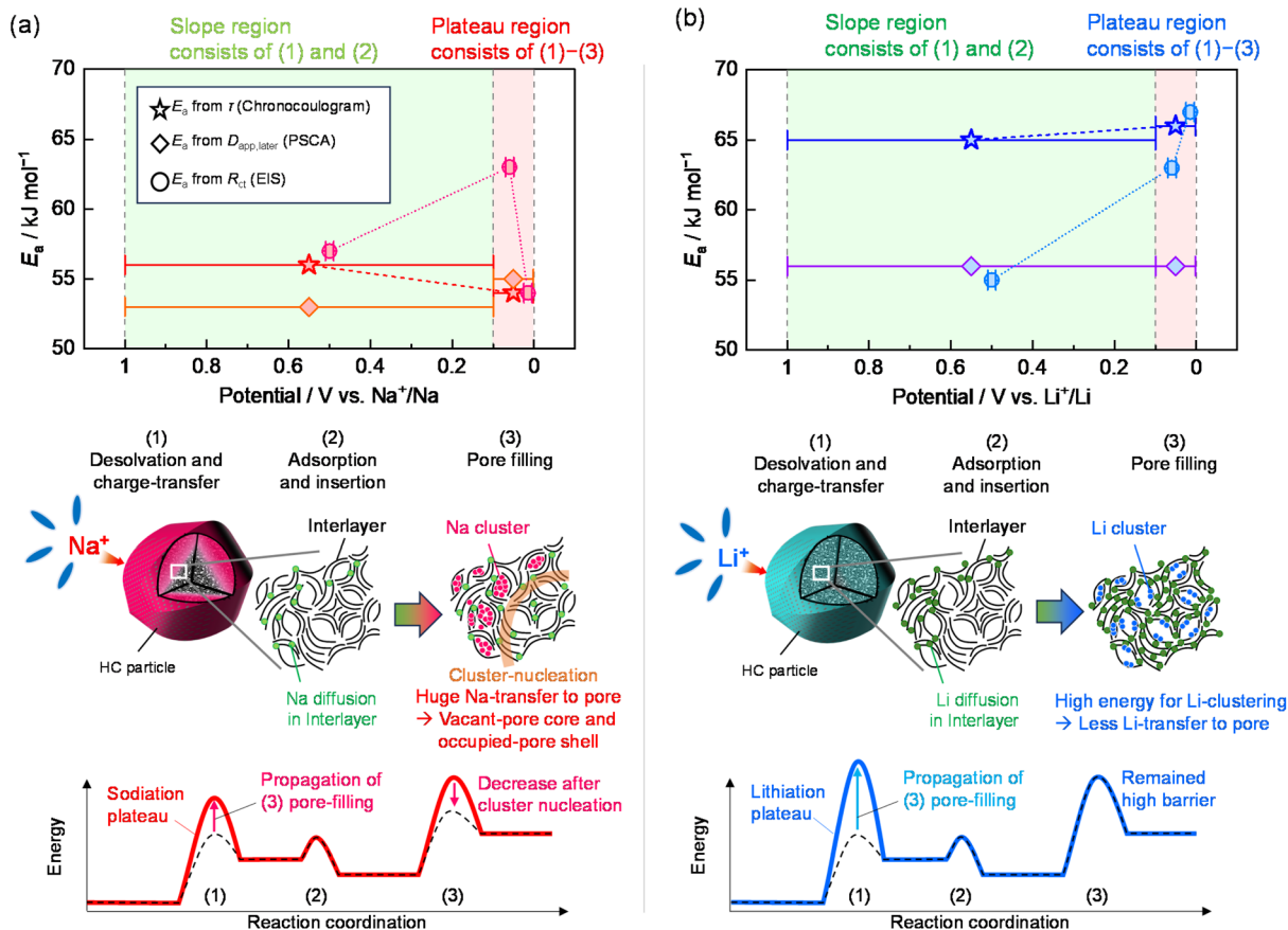
Fig. 9 The summarized results of E_a for (a) sodiation and (b) lithiation of HC from our various measurements; E_a during the insertion process obtained from the \tau of chronocoulogram, D_{app, later} estimated from PSCA, and R_{ct} evaluated by EIS.
