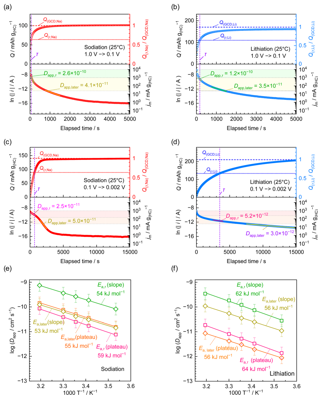
Fig. 6 Chronocouloulograms and corresponding chronoamperograms of 5 vol% HC electrodes for the slope regions of (a) sodiation and (b) lithiation and plateau regions of (c) sodiation and (d) lithiation. The values of D_{\text{app}} were estimated by applying eqn (4), as described in the Experimental section. Activation energies E_{a,\tau} and E_{a,\text{later}} were estimated from D_{\text{app}} vs. T^{-1} plots of D_{\text{app},\tau} and D_{\text{app},\text{later}} during (e) sodiation and (f) lithiation, respectively. The error bars of D_{\text{app}} values are estimated from standard error of the HC particle size.
