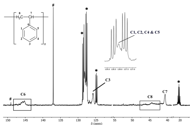
Fig. 2 ^{13}\text{C} NMR (25 ^{\circ}\text{C} , d_8 -toluene, 126 MHz) spectrum of atactic polystyrene prepared using a 0.5 mol% precatalyst loading of 1a and [\text{Ph}_3\text{C}][\text{B}(\text{C}_6\text{F}_5)_4] at room temperature. The resonances are broad and overlapping and have been assigned based on existing literature. 21,30,31 The signals marked as # can be best attributed to unreacted [\text{Ph}_3\text{C}][\text{B}(\text{C}_6\text{F}_5)_4] , remnant toluene or potentially any unreacted styrene. * d_8 -toluene.
