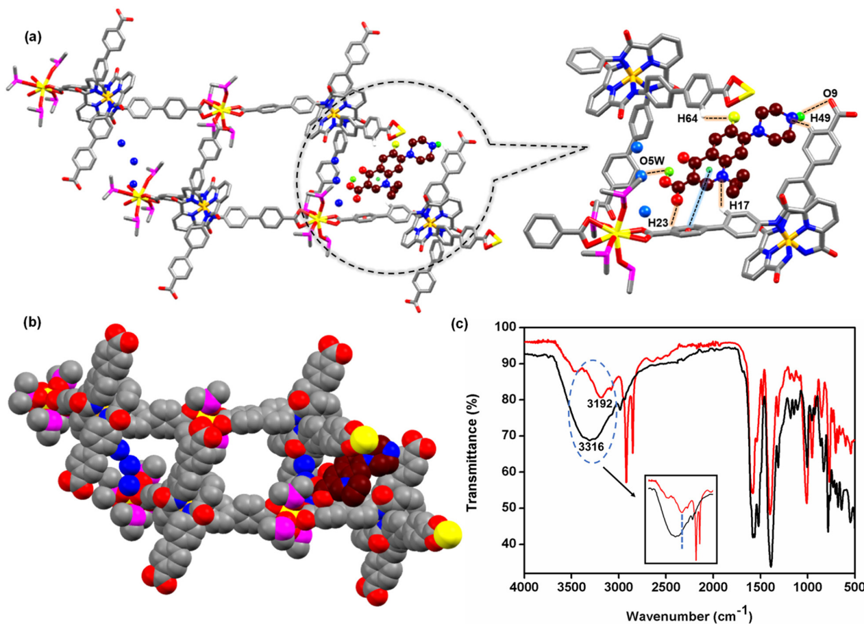
Fig. 6 (a) Molecular docking structure of 1-Tb with CIP, where 1-Tb is shown as a capped-stick model (color code: orange, Co; yellow, Tb; pink, S; blue, N; red, O; grey, C; and white, H), while the CIP molecule is depicted in a ball-and-stick model (color code: olive, F; blue, N; red, O; wine, C; and green, H). H atoms, except for those involved in interactions, have been omitted for clarity. \pi\cdots\pi -stacking interactions are shown by the blue dots, whereas H-bonding interactions are presented by the red dots. (b) Molecular docking structure in a space-filling mode for 1-Tb with CIP (wine color). (c) FTIR spectra of as-synthesised 1-Tb (black trace) and the impregnated sample of 1-Tb with CIP (red trace).
