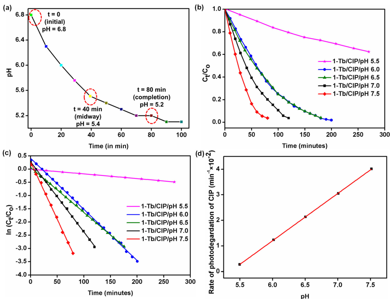
Fig. 4 (a) Plot for the variation of pH with irradiation time for the photocatalytic degradation of CIP using 1-Tb. (b) Photocatalytic activity of 1-Tb for the degradation of CIP at different pH values. (c) Plot of \ln(C_t/C_0) versus time representing the first-order kinetics for the degradation of CIP using 1-Tb at different pH values. (d) Plot for the rate of photodegradation of CIP catalyzed by 1-Tb as a function of pH.
