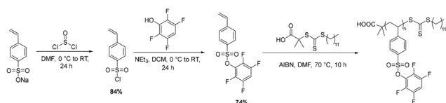
Scheme 2 Synthesis of TFPSS monomer and subsequent RAFT Polymerization. Final polymer M_n (SEC) = 33 kDa, D = 1.40.
