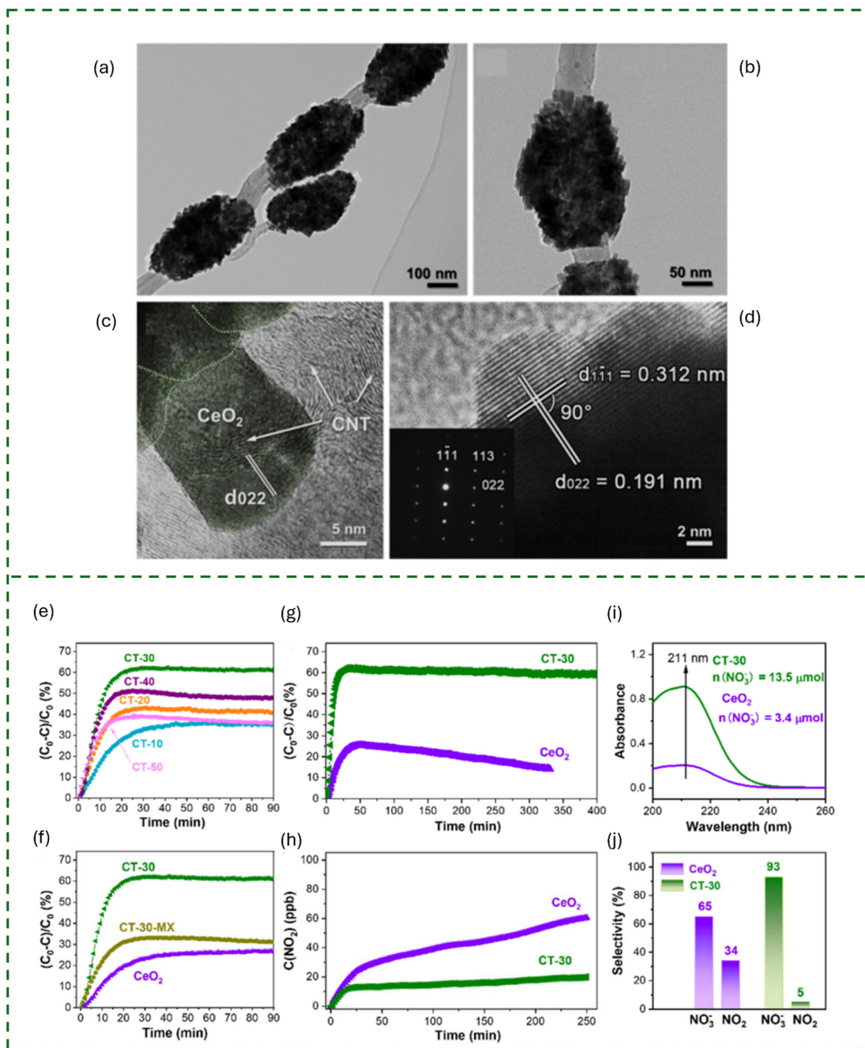
Fig. 13 (a, b) TEM images and (c, d) HRTEM images of CT-30 (the SAED pattern in the inset). Photocatalytic NO oxidation performance of (e) CT-series samples with different CNT contents and (f) \text{CeO}_2 , CT-30, and CT-30-MX, (g) long-term stability test and (h) concentration profiles of \text{NO}_2 during the photocatalytic NO oxidation applying \text{CeO}_2 and CT-30 as catalysts, (i) liquid UV-vis spectra of the catalyst-washed solution after photocatalytic reaction for 250 min, and (j) selectivity of \text{NO}_3^- and \text{NO}_2 for NO oxidation reactions. 173 Figures a–j reprinted from ref. 173 ACS Appl. Nano Mater. , 2022, 5, 3581–3590, with permission from the American Chemical Society, copyright 2026.
