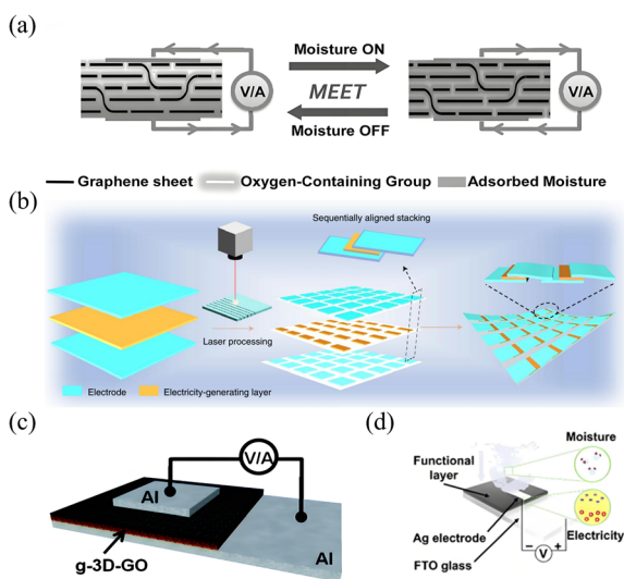
Fig. 6 (a) Schematic illustration of a MEET cycle. 8 Reproduced from ref. 8 with permission from John Wiley and Sons, copyright 2015. (b) Schematic illustration of large-scale integration of HMEG units by sequentially aligned stacking strategy. 16 Reproduced from ref. 16 with permission from Springer Nature, copyright 2021. (c) Schematic illustration of a prototype CPEh based on g-3D-GO that is sandwiched by aluminium electrodes. 11 Reproduced from ref. 11 with permission from Royal Society of Chemistry, copyright 2016. (d) Structure illustration of MEG device. 5 Reproduced from ref. 5 with permission from Elsevier, copyright 2022.
