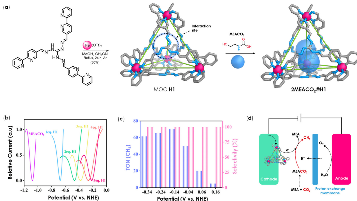
Fig. 5 (a) Schematic process of self-assembly to produce H1 and the formation of the host–guest 2\text{MEACO}_2@ \text{H1} adduct. (b) Square wave voltammetry (SWV) of the systems containing \text{MEACO}_2 (0.1 mM) at different concentrations of H1. (c) Relationship between TON and selectivity for the electrocatalytic reduction of \text{CO}_2 to \text{CH}_4 by H1 at different controlled potentials. (d) Schematic diagram of the cavity-mediated mechanism for the conversion of \text{MEACO}_2 into \text{CH}_4 within tetrahedron H1. Parts (b–d) adapted from ref. 60, https://doi.org/10.1039/d5qi00756a . Copyright 2025, The Royal Society of Chemistry.
