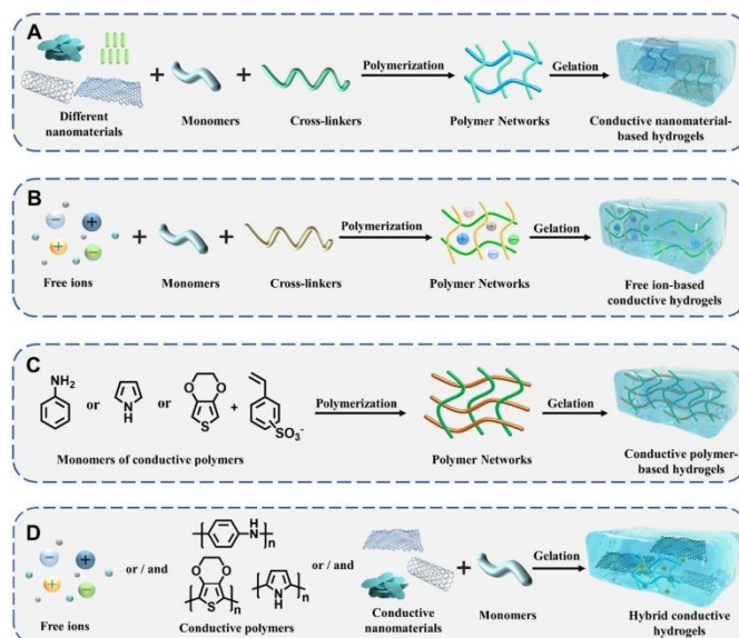
Fig.3. Schematic illustration of the fabrication of conductive hydrogels incorporating different types of conductive fillers: (A) conductive nanomaterials, (B) free ions, (C) conductive polymers, and (D) hybrid conductive systems. This figure has been reproduced from ref.68 with permission from Springer Nature, copyright 2024.
