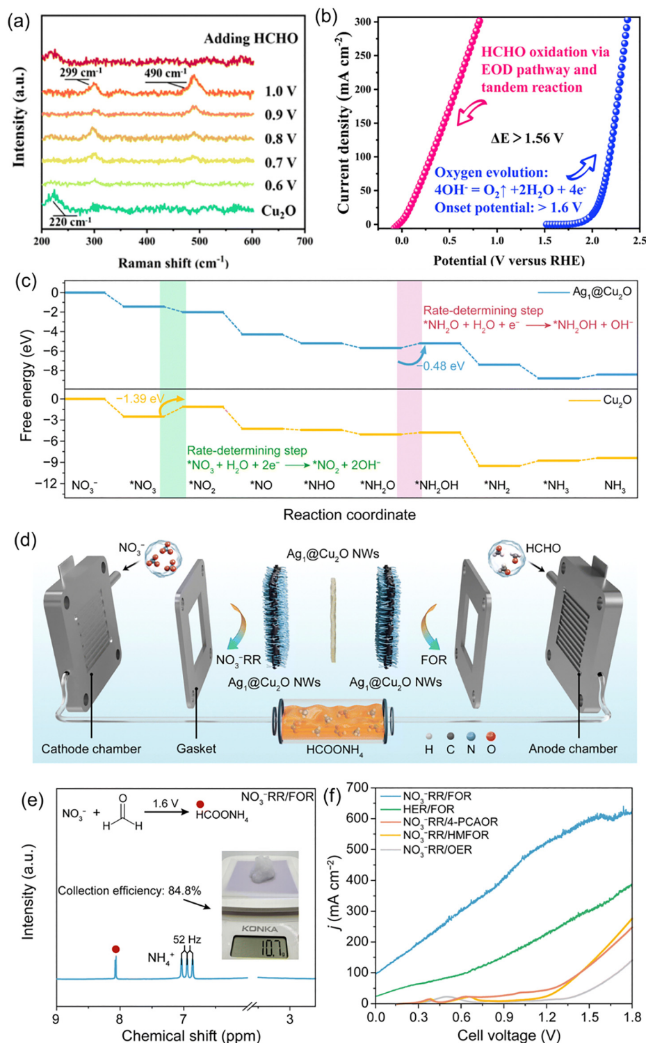
Fig. 18 (a) In situ Raman spectroscopy of \text{Cu}_2\text{O} after holding various potentials from 0.6 V to 1.0 V for 100 s without HCHO and finally adding HCHO. (b) HCHO oxidation over \text{Cu}_2\text{O} and OER over Pt. 18 Reproduced from ref. 18, with permission from The Royal Society of Chemistry, Copyright [2023]. (c) Gibbs free energy diagrams of \text{NO}_3^- RR on \text{Ag}_1@/\text{Cu}_2\text{O} and \text{Cu}_2\text{O} . (d) Schematic illustration of the configuration of the MEA electrolyzer. (e) ^1\text{H} NMR spectrum of the \text{HCOONH}_4 product; inset is a photograph of the 10.7 g of \text{HCOONH}_4 solid isolated. (f) Performance of MEA-based electrolysis for the \text{NO}_3^- RR/OER, \text{NO}_3^- RR/FOR, \text{NO}_3^- RR/4-PCAOR and \text{NO}_3^- RR/HMFOR pairs. 76 Reproduced from ref. 76, with permission from The Royal Society of Chemistry, Copyright [2025].
