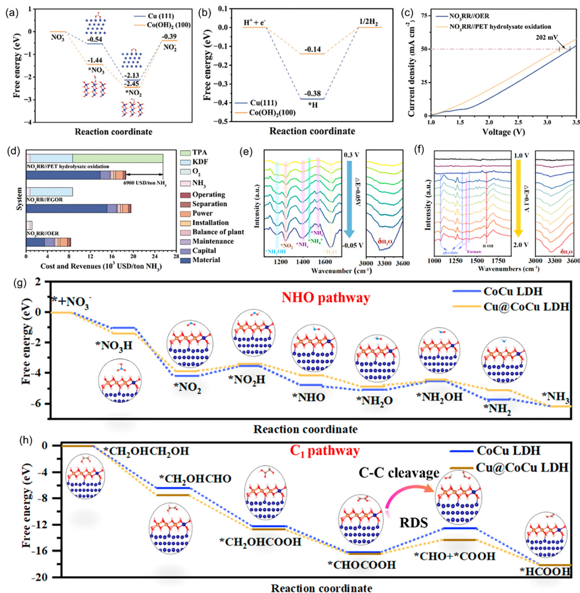
Fig. 19 Free energy profiles (a) for \text{NO}_3^- to \text{NO}_2^- and (b) for the HER on Cu and \text{Co(OH)}_2 . (c) LSV curves of \text{NO}_3\text{RR}||\text{PET hydrolysate oxidation} and \text{NO}_3\text{RR}||\text{OER} . (d) Technoeconomic analysis of \text{NO}_3\text{RR}||\text{OER} , \text{NO}_3\text{RR}||\text{EGOR} and \text{NO}_3\text{RR}||\text{PET hydrolysate oxidation} (USD/tonne \text{NH}_3 ). 54 Reproduced from ref. 54, with permission from John Wiley & Sons, Copyright [2025]. The operando FTIR spectra of the (e) \text{NO}_3^- reduction reaction and (f) of the EG oxidation reaction for the Cu@CoCu LDH. The Gibbs free energy diagrams of the (g) \text{NO}_3\text{RR} and (h) EGOR on both the CoCu LDH and Cu@CoCu LDH. The insets are the corresponding adsorbed structures of different intermediates. 19 Reproduced from ref. 19, with permission from American Chemical Society, Copyright [2024].
