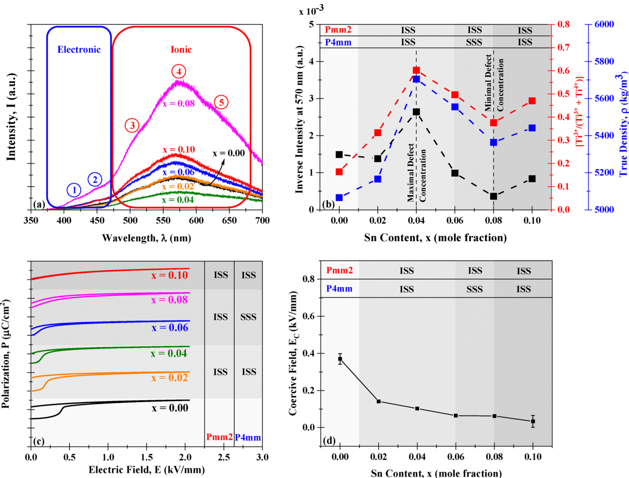
Fig. 4 (a) Photoluminescence spectra, (b) variation in inverse 570 nm intensity, true density and \frac{Ti^{3+}}{[Ti^{3+} + Ti^{4+}]} as a function of Sn^{4+} doping level, (c) unipolar polarization curves (vertically offset) measured at 2.0 \text{ kV mm}^{-1} , and (d) variation in coercive field, E_C as a function of Sn^{4+} doping level for (Ba_{0.85}Ca_{0.15})[(Ti_{0.92-x}Sn_x)Zr_{0.08}]O_3 ( x = 0.00-0.10 ).
