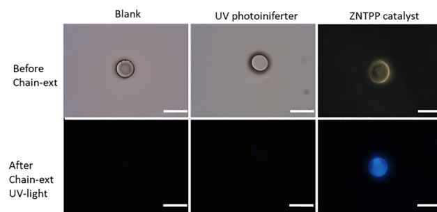
Fig. 9 Microscope images of printed pillars before chain extension (top row) and after chain extension (Bottom row). The white size indicator bar represents 100 \mu\text{m} . UV light was used to initiate the photoiniferter chain extension and on the blank, while green light was irradiated on the ZnTPP containing mixture. The experiments were performed with BuMA with 5 wt% 1-pyrene methylacrylate in DMSO. Only after the catalysed reaction, the sample shows fluorescence indicating attachment of the pyrene moiety.
