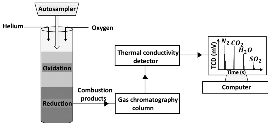
Fig. 10 Simplified diagram of CHNS elemental analyzer, where the sample is combusted, the resulting gases are separated by a gas chromatography column eluting to a thermal conductivity detector.
