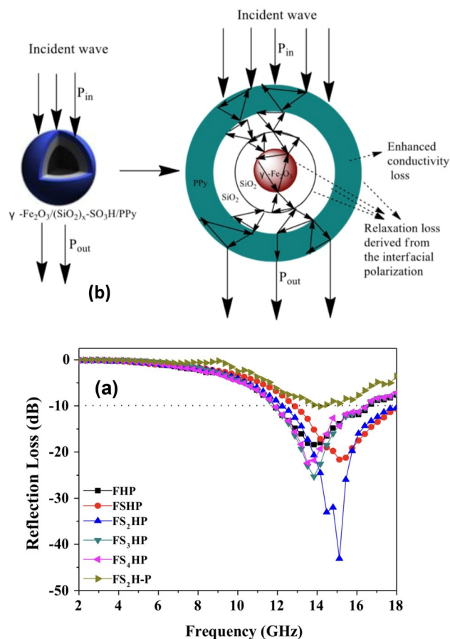
Fig. 22 (a) Variation of R_L of \gamma-Fe_2O_3/(SiO_2)_x-SO_3H/polypyrrole (referred to as FS_xHP , where x = 0.1, 1, 2, 3, 4 ) core/shell/shell microspheres and FS_2H-P (physical blend of FS_2H and PPy) with the frequency ( d = 2 mm), and (b) physical model of the effects of core/shell/shell structures on the microwave absorption. 390 Reproduced with permission from Springer.
