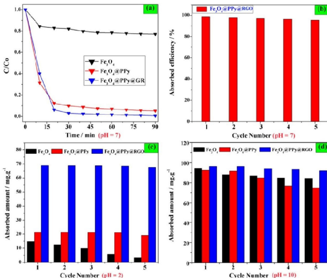
Fig. 35 (a) Removal efficiency of magnetic adsorbents in neutral solution (pH 7); (b) removal efficiency of Fe_3O_4@PPy@RGO in five cycles, neutral solution (pH 7); (c) removal efficiency of magnetic adsorbents in acidic solution (pH 2) and (d) alkaline solution (pH 10). 529 Reproduced with permission from Elsevier.
