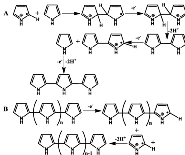
Fig. 6 The formation of dimer and trimer of pyrrole (A) and further formation of the PPy (B). 128 Reproduced with permission from Elsevier.
