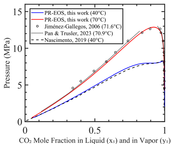
Fig. 11 Benchmarking of PR-EOS-predicted phase envelopes in this work for the \text{CO}_2 - n -decane system against experimental data from Jiménez-Gallegos et al. 103 at 71.6\text{ }^{\circ}\text{C} , and PR-EOS models from Pan and Trusler 94 and Nascimento et al. 104 at 40 and 70.9\text{ }^{\circ}\text{C} . The present model shows good agreement across the full two-phase region.
