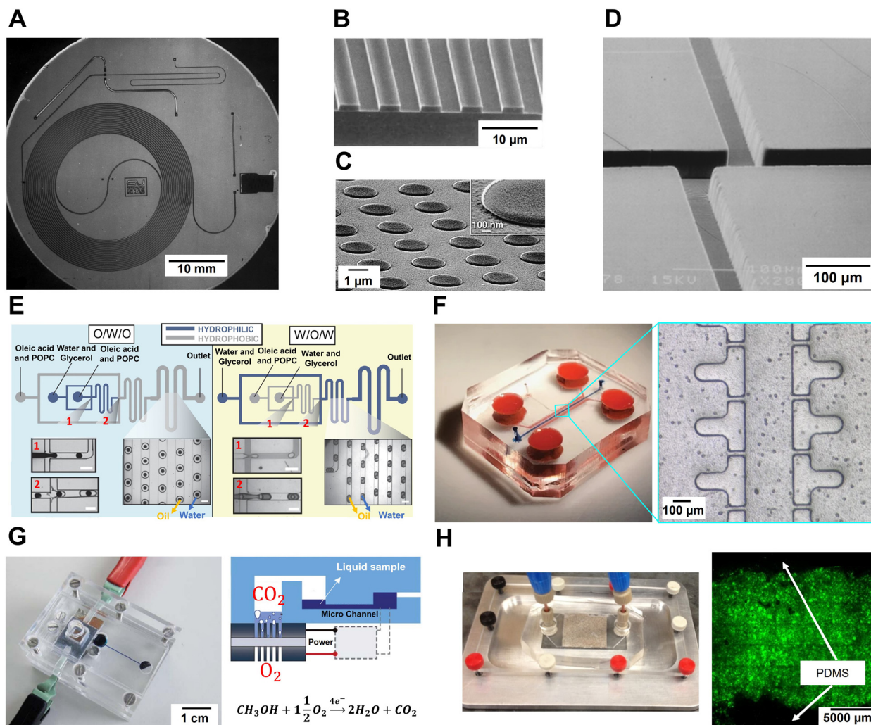
Fig. 1 Microfabricated chips for fluidic applications: (A) the first miniaturized gas chromatograph fabricated on silicon wafer fabricated by Terry et al. , 38 1979 (adapted with permission from de Mello. 39 Copyright © 2002 the Royal Society of Chemistry). (B) Rectangular pattern of PDMS slabs fabricated by micro-molding in capillaries on a gold film (adapted with permission from Kim et al. 40 Copyright © 1995 Nature Publishing Group). (C) SEM image of circular patterns on silicon wafer fabricated by microcontact printing (adapted with permission from Marzolin et al. 41 Copyright © 1998 Elsevier). (D) SEM image of a double T-section pattern on PDMS fabricated by replica molding (adapted with permission from Duffy et al. 42 Copyright © 1998 American Chemical Society). (E) Surface modification (plasma treatment and polyvinyl alcohol (PVA) deposition) of PDMS microfluidic channels to apply varied wettability to generate oil in water in oil (O/W/O) and water in oil in water (W/O/W) double emulsions. All scale bars are 300 μm (adapted from Trantidou et al. 43 under CC-BY License). (F) PDMS cartilage-on-a-chip with T-shaped pillars fabricated to predict the efficacy of disease-modifying osteoarthritis (DMOA) drugs (adapted with permission from Occhetta et al. 44 Copyright © 2019 Nature Publishing Group). (G) PDMS micro direct methanol fuel cell (μDMFC)-micropump where methanol oxidation produces CO 2 to pressurize the liquid sample toward the analysis (adapted with permission from Esquivel et al. 45 Copyright © 2012 the Royal Society of Chemistry). (H) Real rock-microfluidic flow cell (RR-MFC) configuration where a thin section (500 μm thickness) of the sandstone sample is assembled with a PDMS channel to involve geochemical reactions in visualizing fluid flow in subsurface porous rocks. On the right, displacement of fluorescein-carrying fluid with dye-free fluid in the RR-MFC chip (adapted with permission from Singh et al. 46 Copyright © 2017 Elsevier).
