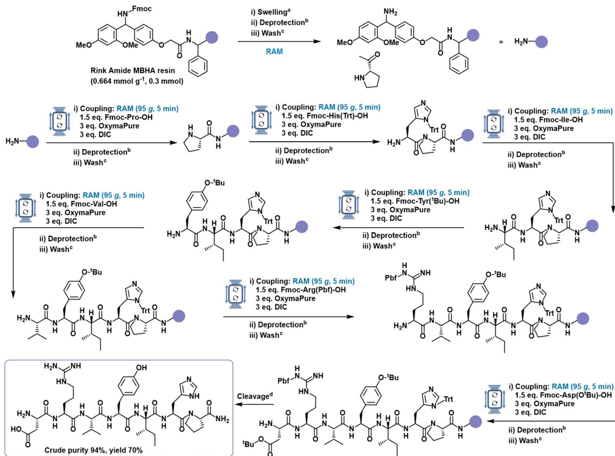
Fig. 4 Reaction conditions for the synthesis of heptapeptide Angiotensin (1–7) (Asp–Arg–Val–Tyr–Ile–His–Pro). Resin: Fmoc Rink Amide MBHA (loading 0.664 \text{ mmol g}^{-1} , 0.3 \text{ mmol} scale); a swelling: 4 mL DMF, RAM (80g, 20 min); b deprotection: 4 mL of a solution 20% PIP in DMF, RAM (80g, 5 min) \times 2 ; c wash: 3 mL DMF \times 2 ; coupling: 1.5 eq. AA, 3 eq. DIC, 3 eq. OxymaPure, RAM (95g, 5 min); d cleavage: 10 mL TFA/TIPS/H 2 O (95 : 2.5 : 2.5). Yield (70%), crude purity (94%), as a TFA salt.
