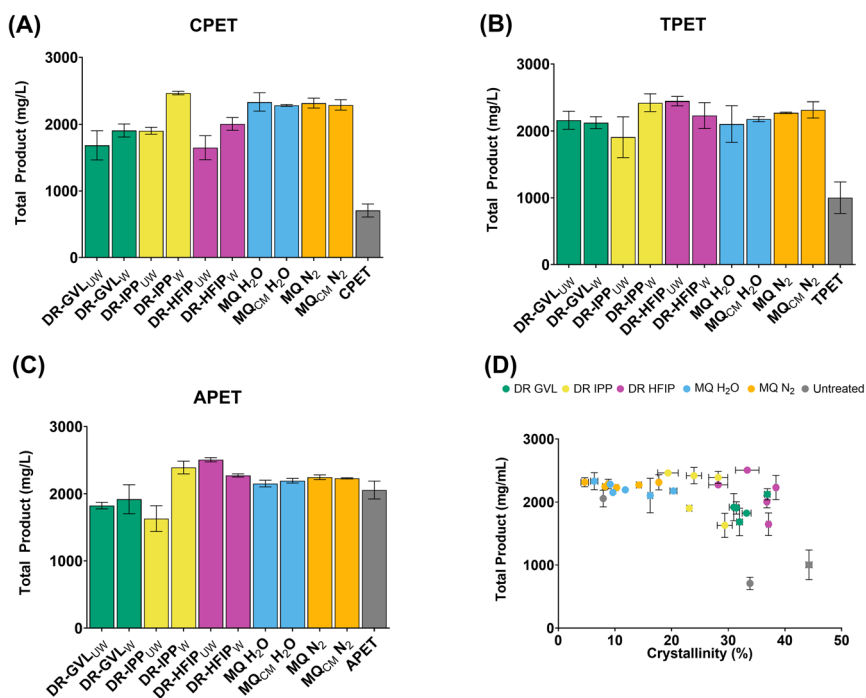
Fig. 2 Activity of LCC ICCG against pre-treated (A) semi-crystalline PET powder (CPET), (B) polyester textile (TPET,) and (C) amorphous PET powder (APET,) substrates. Reactions were carried out in triplicate, with 500 \mu L of 0.5 M potassium phosphate buffer (pH 8.0) containing 500 nM LCC ICCG , at 65 ^{\circ} C for 96 hours with continuous agitation at 300 rpm. Enzyme-free reactions served as negative controls. Degradation products from PET hydrolysis were quantified by HPLC, measuring the release of the monomers TPA, MHET, and BHET. Data are presented as mean \pm standard deviation (SD) of triplicate reactions, UW: unwashed; W: washed; CM: cryo-milling. The relationship between crystallinity and total product yield is shown in panel D, and a weak negative correlation is observed (corr = -0.5 , R squared = 0.27 ).
