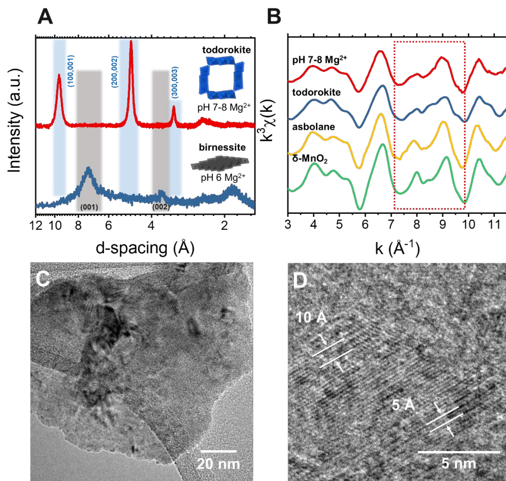
Fig. 1. The formation of todorokite at pH 7–8 in the presence of Mg^{2+} . (A) X-ray diffraction of Mn oxides shows the clear diffractions of todorokite (blue bar) at pH 7–8. At pH 6, only birnessite (or \delta -MnO 2 ) was observed after 6 h reaction. (B) The analysis of extended X-ray absorption fine structure supports the formation of todorokite at pH 7–8. TEM images of the platy show the morphology of poorly crystalline todorokite (C) and the large d-spacing of todorokite (D) prepared at 100 mM Mg^{2+} pH 7–8.
