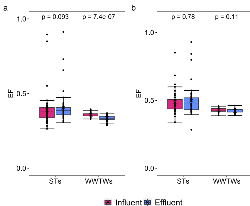
Figure 5: Enantiomeric fraction (EF) of citalopram (a) and desmethylocitalopram (b) in influent and effluent of five community STs ( n = 60 ) 120 and five centralised WWTWs ( n = 35 ) 216 with Wilcoxon results (significant difference for p < 0.05 ).
