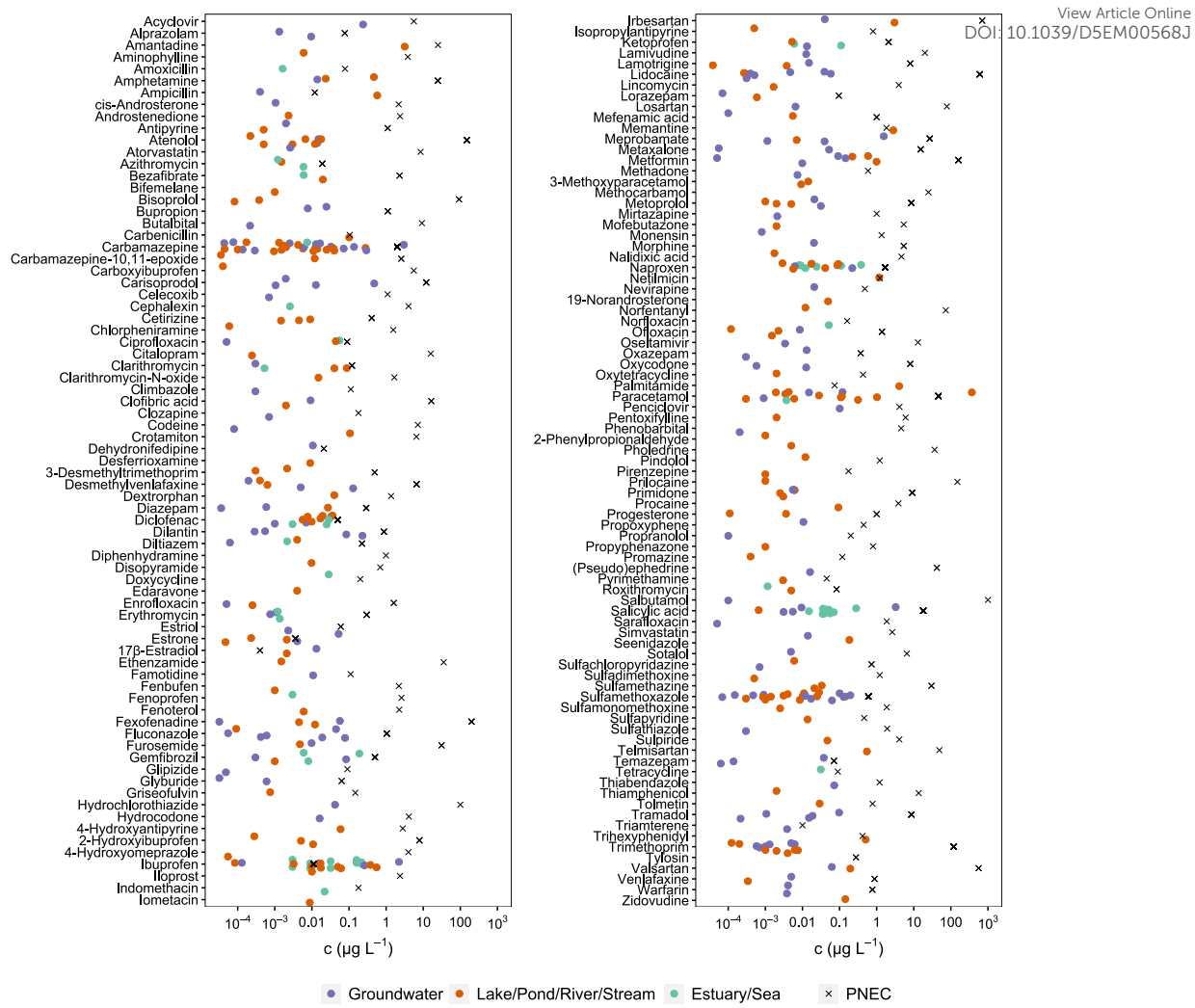
Figure 6: Mean concentration (data from one study, studies in Table 2) and lowest freshwater PNEC 122 of active pharmaceutical ingredients (APIs) in ground- and surface water, including streams, lakes, ponds, canals and seawater, impacted by OWTWs (c in \mu\text{g L}^{-1} ; logarithmic scale). Some locations also receive discharges from centralised WWTWs, but known data points directly downstream of centralised WWTWs were excluded.
