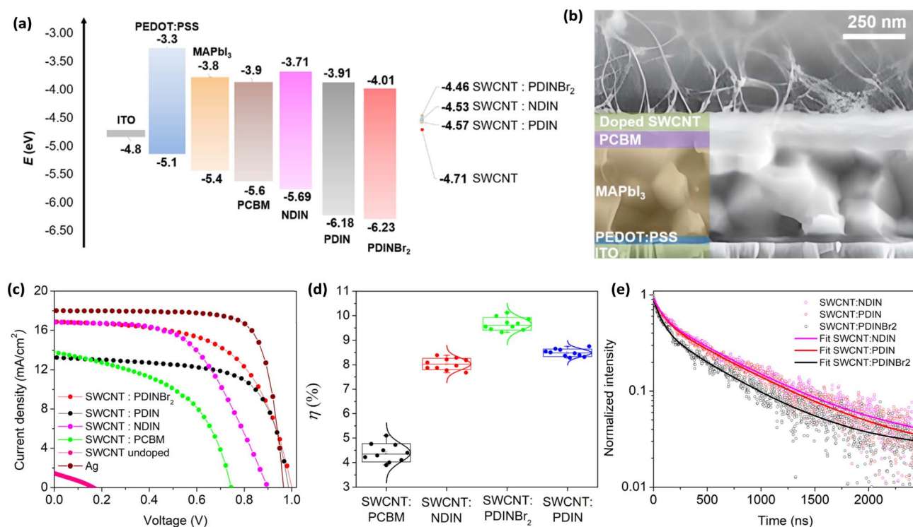
Fig. 4 (a) Energy level diagram of the inverted perovskite solar cell, (b) their cross-sectional SEM image, (c) comparison of J-V characteristics of inverted perovskite solar cells incorporating different cathodes, (d) statistical distributions of power conversion efficiency, and (e) microwave photoconductivity decay ( \mu -PCD) profiles of ITO/MAPbI 3 /PCBM/n-doped SWCNT bilayers.
