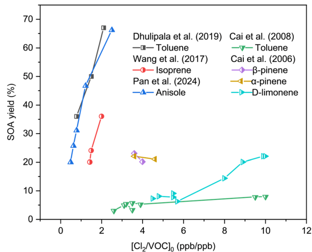
Fig. 5 Influence of [\text{Cl}_2/\text{VOC}]_0 on SOA formation from Cl-initiated VOC oxidation. Data are from Dhulipala et al. (2019), 135 Cai et al. (2008), 42 Wang et al. (2017), 116 Pan et al. (2024), 138 and Cai et al. (2006). 134
