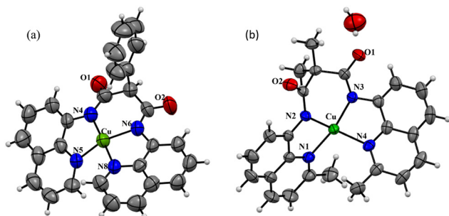
Fig. 1 (a) ORTEP plot of (a) CuL2 (CCDC No. 2491828) and (b) CuL3 (CCDC No. 2477383) shown at the 50% probability level with only heteroatoms bonded. Selective interatomic bond distances and angles for CuL2 : Cu(1)–N(4) = 1.941 Å, Cu(1)–N(5) = 2.015 Å, Cu(1)–N(6) = 1.941 Å, Cu(1)–N(8) = 1.989 Å, [N(4)–Cu(1)–N(5)] = 83.0°, [N(4)–Cu(1)–N(6)] = 98.7°, [N(4)–Cu(1)–N(8)] = 172.9°, [N(5)–Cu(1)–N(6)] = 159.3°, [N(5)–Cu(1)–N(8)] = 97.7°, [N(6)–Cu(1)–N(8)] = 83.2°. CuL3 : Cu(1)–N(1) = 1.997 Å, Cu(1)–N(2) = 1.912 Å, Cu(1)–N(6) = 2.003 Å, Cu(1)–N(8) = 1.914 Å, [N(1)–Cu(1)–N(2)] = 83.6°, [N(1)–Cu(1)–N(4)] = 105.9°, [N(1)–Cu(1)–N(3)] = 156.4°, [N(2)–Cu(1)–N(4)] = 148.0°, [N(2)–Cu(1)–N(3)] = 98.4°, [N(4)–Cu(1)–N(3)] = 84.9°.
