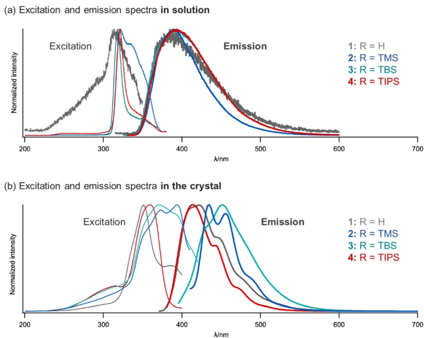
Fig. 4 Excitation and emission spectra of 1–4 in (a) dilute chloroform solutions (concentration: 10^{-3}\text{ mol L}^{-1} for both spectra) and (b) the crystalline state.
