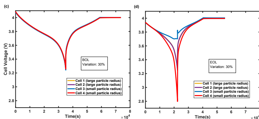
Fig. 11: Cell voltage profiles for four cells in a battery pack with a 2S2P electrical configuration for 10% and 30% particle radius variation, cycled at 0.1C under 3.25–4.0 V. Panels (a, b) display the BOL and EOL voltage profiles, respectively, for the 10% variation case. Panels (c, d) display the corresponding BOL and EOL voltage profiles for the 30% variation case
