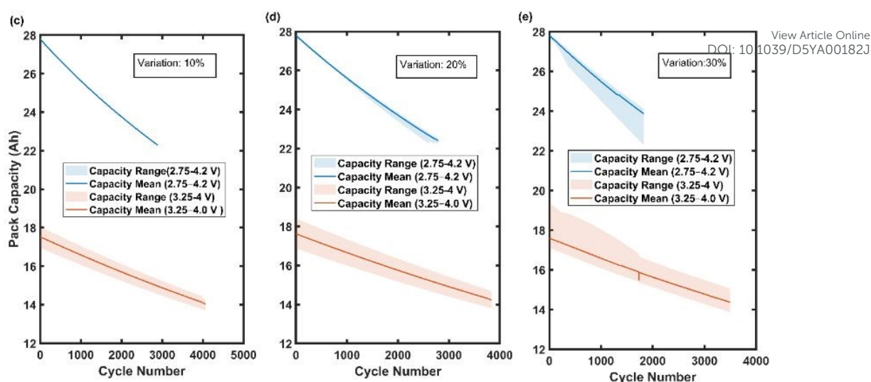
Fig. 7: Capacity Analysis of Series-Connected Cells. Panels (a, b): Spread of cumulative SEI capacity loss across cells under 2.75-4.2 V and 3.25-4 V; panels (c-e) show the degradation of pack capacity under both voltage windows for 10%, 20%, and 30% variation, respectively.
