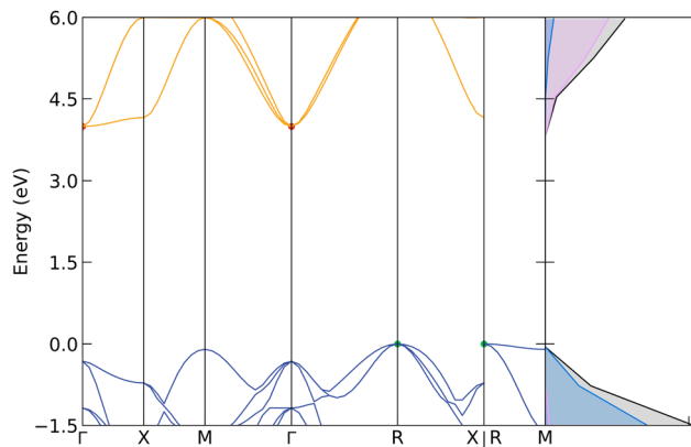
(a) Pm\bar{3}m
