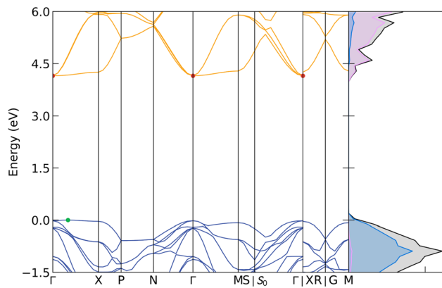
(b) I4/mcm
