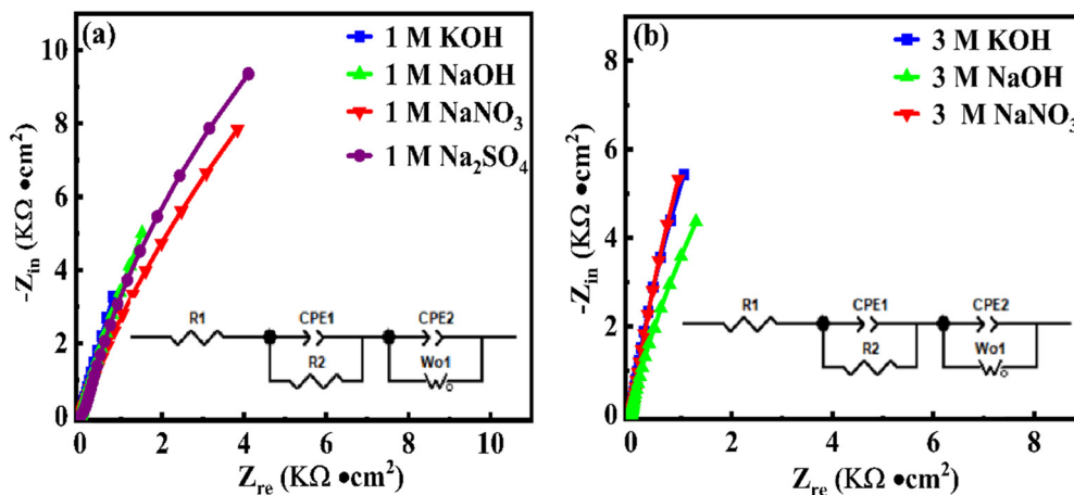
Fig. 19 Nyquist plots of \text{Mn}_2\text{O}_3\text{-9} in (a) 1 M and (b) 3 M concentrations of different electrolytes. The insets are the equivalent circuits.
