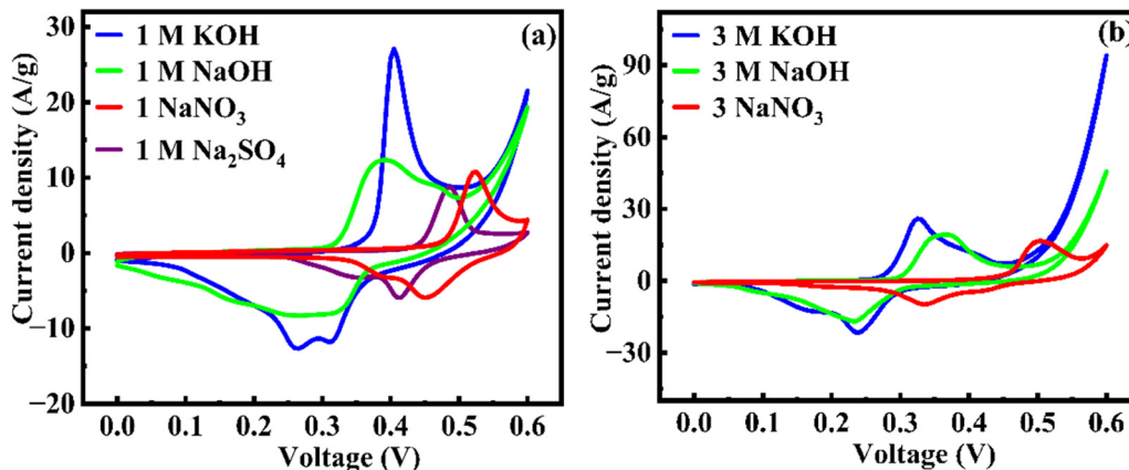
Fig. 8 Cyclic voltammograms of \text{Mn}_2\text{O}_3\text{-9} in (a) 1 M and (b) 3 M concentrations of different electrolytes.
