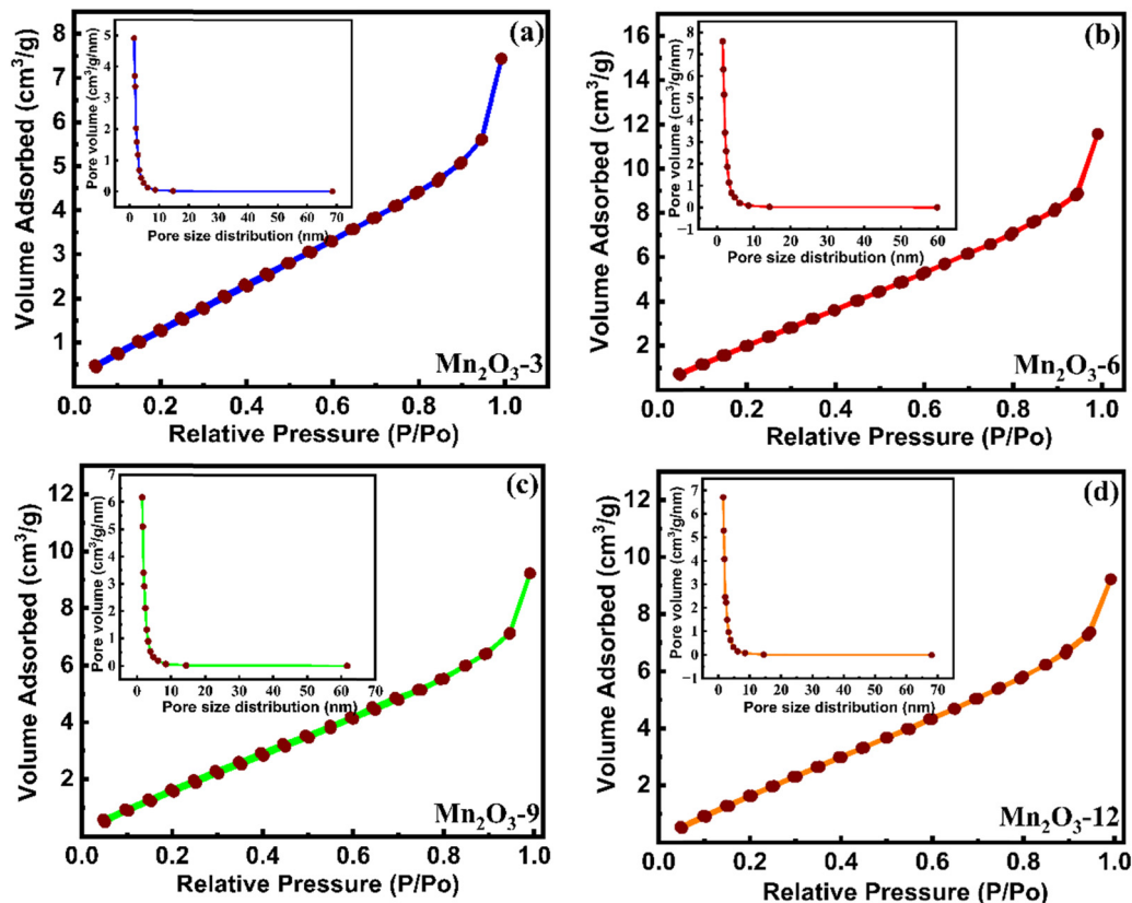
Fig. 4 (a)–(d) N_2 adsorption and desorption plots of the Mn_2O_3 particles measured at 77 K. The inset shows pore size distribution.
