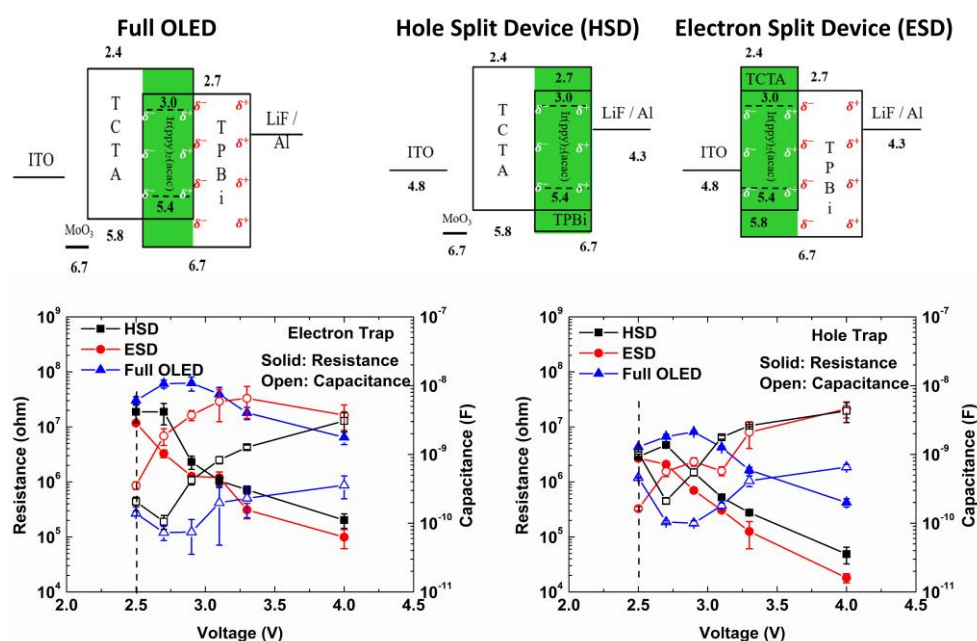
Fig. 13 Energy-level diagrams of the fabricated devices (Full OLED, HSD and ESD) and the simulated trapped electrons and holes in the dopant of the EML. Reproduced with permission from Ref. 37 Copyright 2023, Elsevier Ltd.
