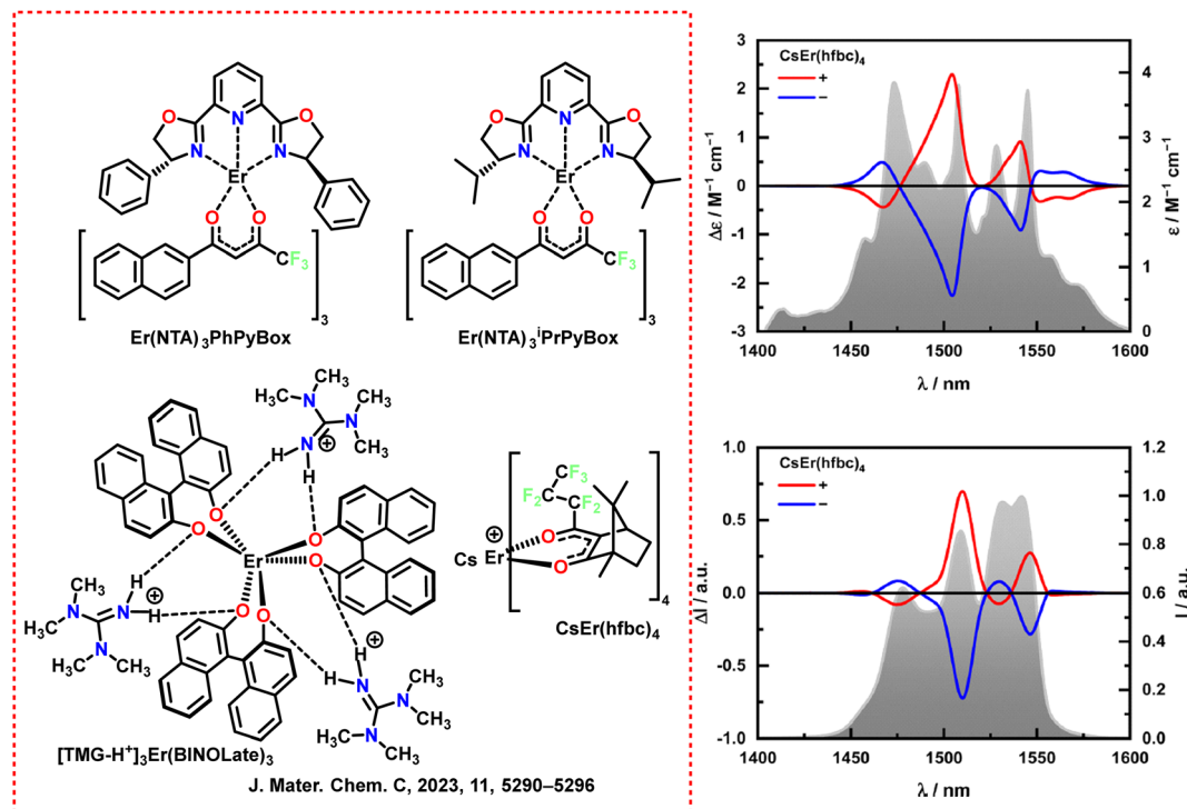
Scheme 50 (Left) Chemical structures of the ligands and Ln complexes ( \text{CsEr}(\text{hfbc})_4 , [\text{TMG-H}^+]_3\text{Er}(\text{BINOLate})_3 , and \text{Er}(\text{NTA})_3\text{PrPyBox} ), adapted from ref. 98. (Right) (Top) NIR-CD spectra of \text{CsEr}(\text{hfbc})_4 (16 mM) with average total absorption traced in the background (in grey). (Bottom) NIR-CPL spectra of \text{CsEr}(\text{hfbc})_4 (1 mM) with normalised average total emission traced in the background (in grey). Reproduced from ref. 98 with permission from the Royal Society of Chemistry, copyright [2023]. 98
