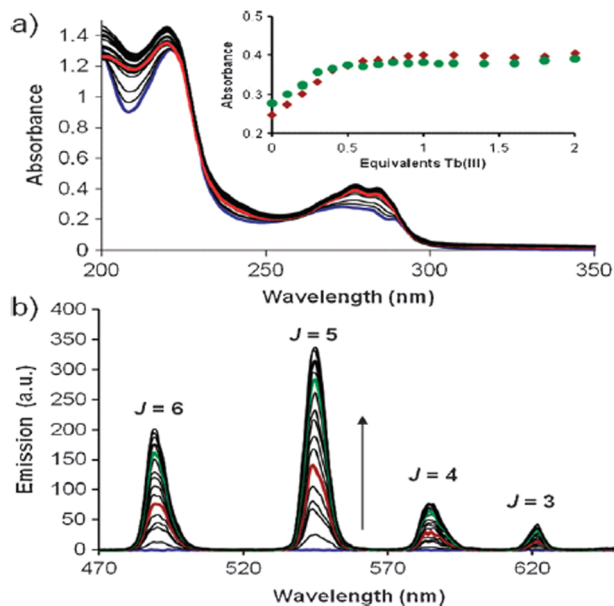
Scheme 20 (Above) Chemical structures of ligands 1 and 2. 75 (Below) (a) Changes in the UV-vis absorption spectrum of 1 (upon titration with Tb(CF 3 SO 3 ) 3 ) in CH 3 CN. Inset: The changes at 275 nm for 1 2 Tb and 2 2 Tb. (b) Corresponding changes in Tb(III) emission. Reproduced from ref. 75 with permission from the Royal Society of Chemistry, copyright [2011]. 75
