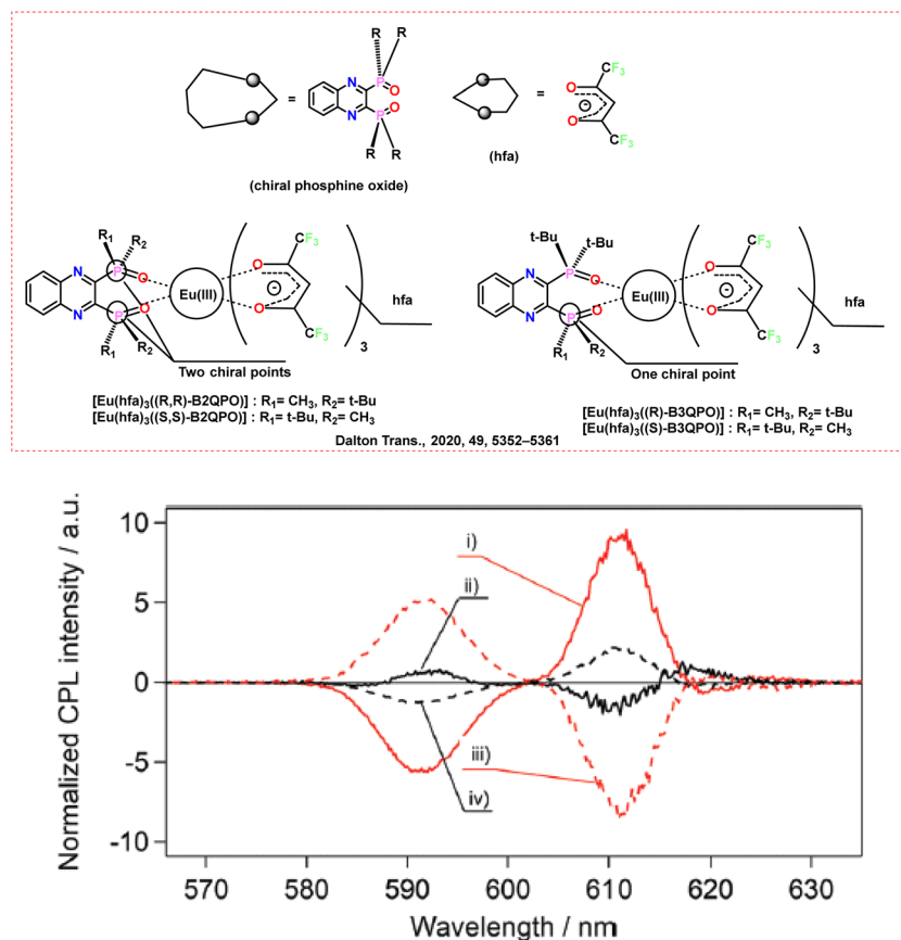
Scheme 32 (Above) Chemical structures of the ligands and Ln complexes [Eu(hfa) 3 ((R,R)/(S,S)-B2QPO)] and [Eu(hfa) 3 ((R)/(S)-B3QPO)]. 82 (Below) CPL spectra of [Eu(hfa) 3 ((R,R)-B2QPO)] ((i), red solid line), [Eu(hfa) 3 ((R)-B3QPO)] ((ii), black solid line), [Eu(hfa) 3 ((S,S)-B2QPO)] ((iii), red dashed line) and [Eu(hfa) 3 ((S)-B3QPO)] ((iv), black dashed line) in dichloromethane. Reproduced from ref. 82 with permission from the Royal Society of Chemistry, copyright [2020]. 82
