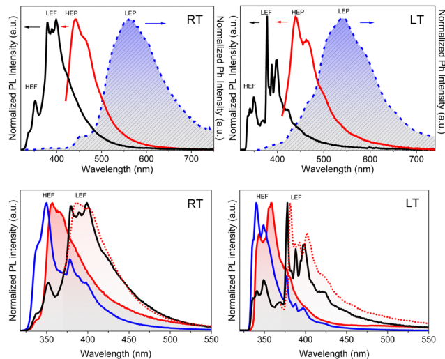
Fig. 30 Normalized emission at 298 K (left) and 77 K (right). Top: TT-(N)-CzM crystals: PL spectra (continuous lines): \lambda_{\text{exc}} = 300 nm (black) and \lambda_{\text{exc}} = 400 nm (red); delayed spectra (blue dashed): delay 1 ms, window 5 ms. Bottom: PL emission spectra of: TT-(N)-CzM crystals, \lambda_{\text{exc}} = 300 nm (red continuous); \lambda_{\text{exc}} = 355 nm (red dotted); TT-(N)-CzT crystals, \lambda_{\text{exc}} = 300 nm, before (black) and after (blue) grinding.
