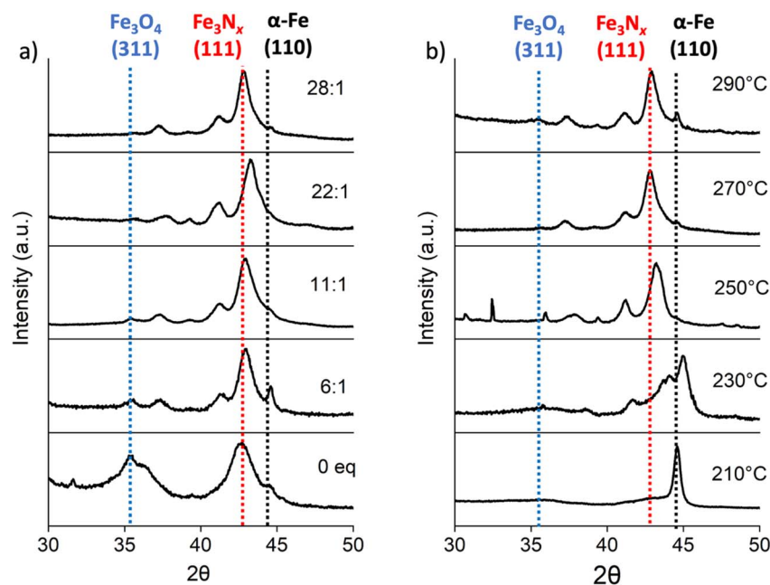
Fig. 4 Powder XRD patterns of nanoparticles obtained from (NEt 4 )[Fe 4 N(CO) 12 ] showing (a) effects of urea concentration and (b) effects of temperature. The reference lines: \epsilon -Fe 3 N (111) in red, \alpha -Fe (110) in black, and iron oxide (311) in blue. The increase in (a) the relative proportion of urea or (b) the reaction temperature shifts primary phase from \alpha -Fe and iron oxide to \epsilon -Fe 3 N.
