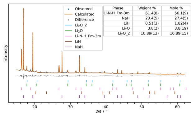
Fig. 7 Observed-calculated-difference (OCD) profile plot from the 1-11 Rietveld refinement of the solvothermal Fm\bar{3}m Li–N–H and NaH phases, note that the increased percentages of \text{Li}_2\text{O}_2 is attributed to exposure during sample transportation.
