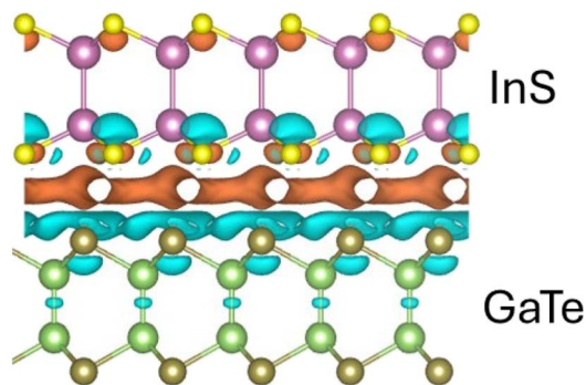
Fig. 8 The charge density difference of the InS/GaTe heterostructure: pink, yellow, green, and brown balls are In, S, Ga, and Te atoms, respectively. The orange and cyan iso-surfaces represent charge accumulation and depletion, respectively. The iso-surface scaling is set to 7.9 \times 10^{-5} e/a_0^3 .
