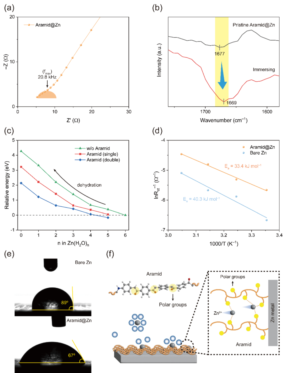
Fig. 3 (a) Enlarged EIS plot of Aramid@Zn symmetric cells. (b) FT-IR spectra of the aramid layer with/without immersing in 2 M ZnSO 4 electrolyte for 24 h. The spectra were shown in the range of 1600–1700 cm -1 to indicate the variation of C=O. (c) Relative energy of hydrated Zn(H 2 O) n complex with and without aramid chains in reference to the fully hydrated state ( n = 6 ). (d) The activation energy of Bare Zn and Aramid@Zn anodes. (e) Contact angles of 2 M ZnSO 4 electrolyte on the Bare Zn and Aramid@Zn anodes. (f) Schematic illustration of ion-transport process in aramid polymer coating.
