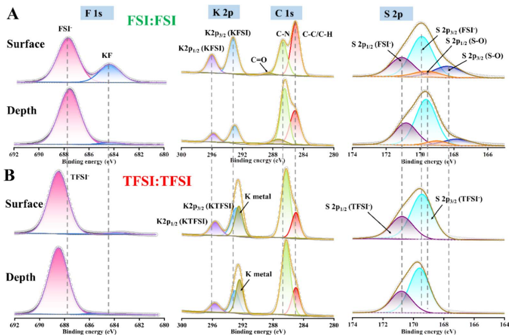
Fig. 6 XPS of the K metal surface and bulk (depth of 8 nm, Ar + etching speed of 0.8 nm min -1 ) after immersing for 28 days in (A) KFSI:Pyr 120 FSI or (B) KTFSI:Pyr 120 TFSI solutions (the grey open points represent the experimental data, and the solid lines represent the fitting results).
