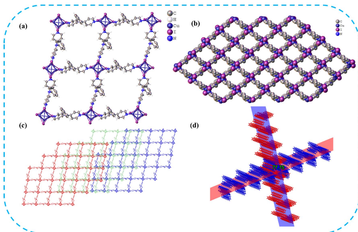
Fig. 1 (a) 2D sheet of the rhombus grid network of Cu-MOF (b) Space filled model of 2D Cu-MOF . (c) \text{C-H}\cdots\text{I} interactions leading to parallel stacking of sheets. (d) Interpenetration of two sheets.
