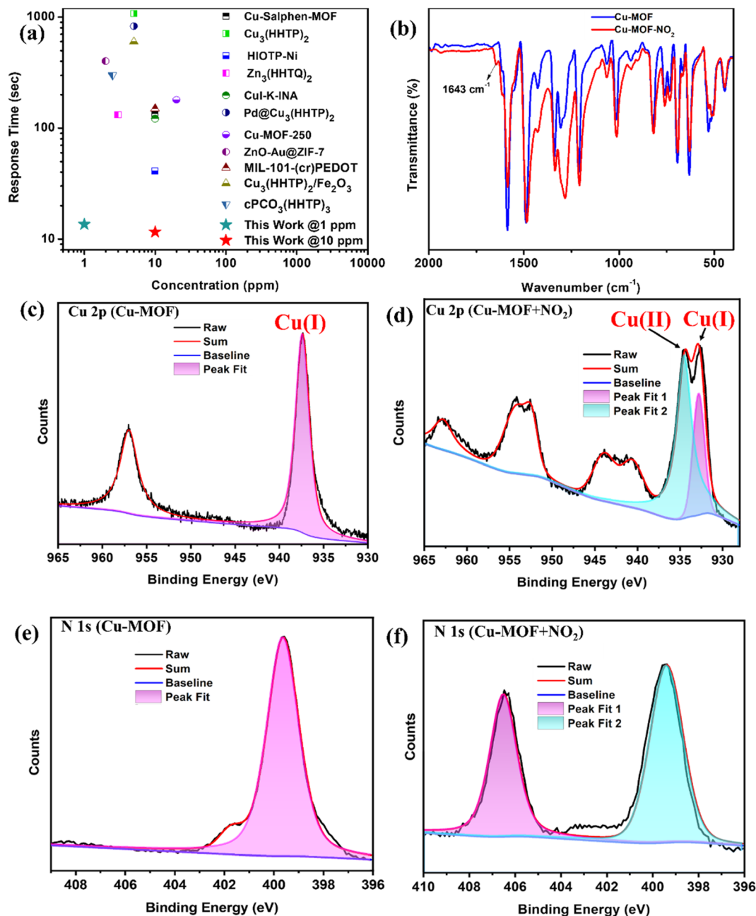
Fig. 4 (a) Response time comparison of the Cu-MOF sensor with the reported MOFs and hybrid MOF-based \text{NO}_2 sensors at room temperature (Tables S2 and S3†). (b) IR-spectra of the Cu-MOF sensor before and after \text{NO}_2 exposure. High-resolution Cu2p XPS spectra (c) before \text{NO}_2 exposure and (d) after \text{NO}_2 exposure; high-resolution N1s XPS spectra (e) before \text{NO}_2 exposure and (f) after \text{NO}_2 exposure.
