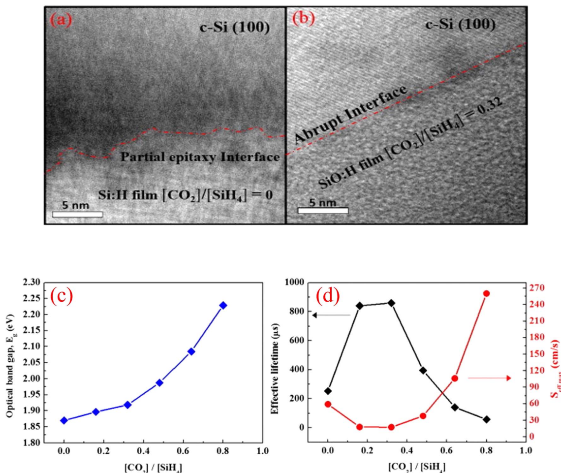
Fig. 8 (a) HRTEM image without CO 2 , a partial epitaxial layer is found between the a-Si:H/c-Si interface, even though the passivation layer provided abundant hydrogen content (b) with CO 2 /CO 2 /[SiH 4 ] = 0.32, the partially epitaxial phase was suppressed and an abrupt interface was formed with excellent surface passivation by terminating the dangling bonds (c) curve of band gap with CO 2 concentration (d) the results of \tau_{eff} and the upper limit of S_{eff} for various ratios of [CO 2 ]/[SiH 4 ], the \tau_{eff} increased and reaches the maximum value of 860 μs ( S_{eff} = 17.4 cm -1 s -1 ) for increasing the ratio of [CO 2 ]/[SiH 4 ] from 0 to 0.32. After the maximum values, \tau_{eff} rapidly decreased with an increasing CO 2 gas flow rate due to the lack of abundant hydrogen content in the a-SiO:H films (reproduced from ref. 81 with permission from Elsevier, copyright 2015).
