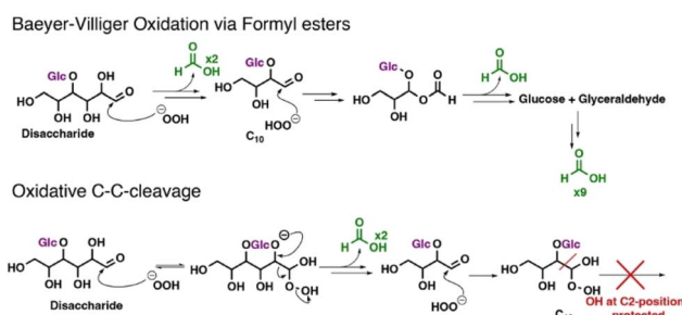
Scheme 1 Possible pathways in the conversion of reducing carbohydrates using alkaline hydrogen peroxide solutions, either via formyl esters or via oxidative C–C cleavage, leading to different anticipated product compositions.
