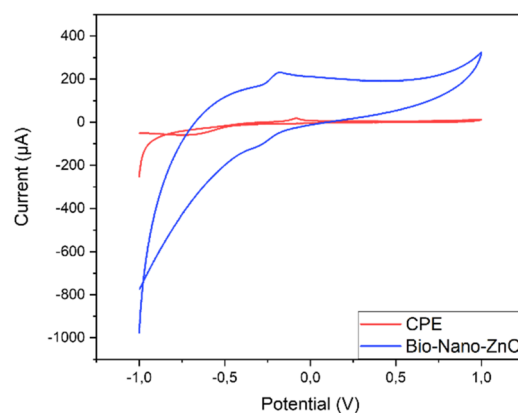
Fig. 6 CV measurements for both the CPE and bio-NPs-ZnO/CPE in 2 \text{ mM} totarolone dissolved in 0.1 \text{ M} NaCl, at a scan rate of 100 \text{ mV s}^{-1} and a start potential of -1.0 \text{ V} vs. \text{Hg}/\text{Hg}_2\text{Cl}_2 , \text{KCl}/\text{sat} .
