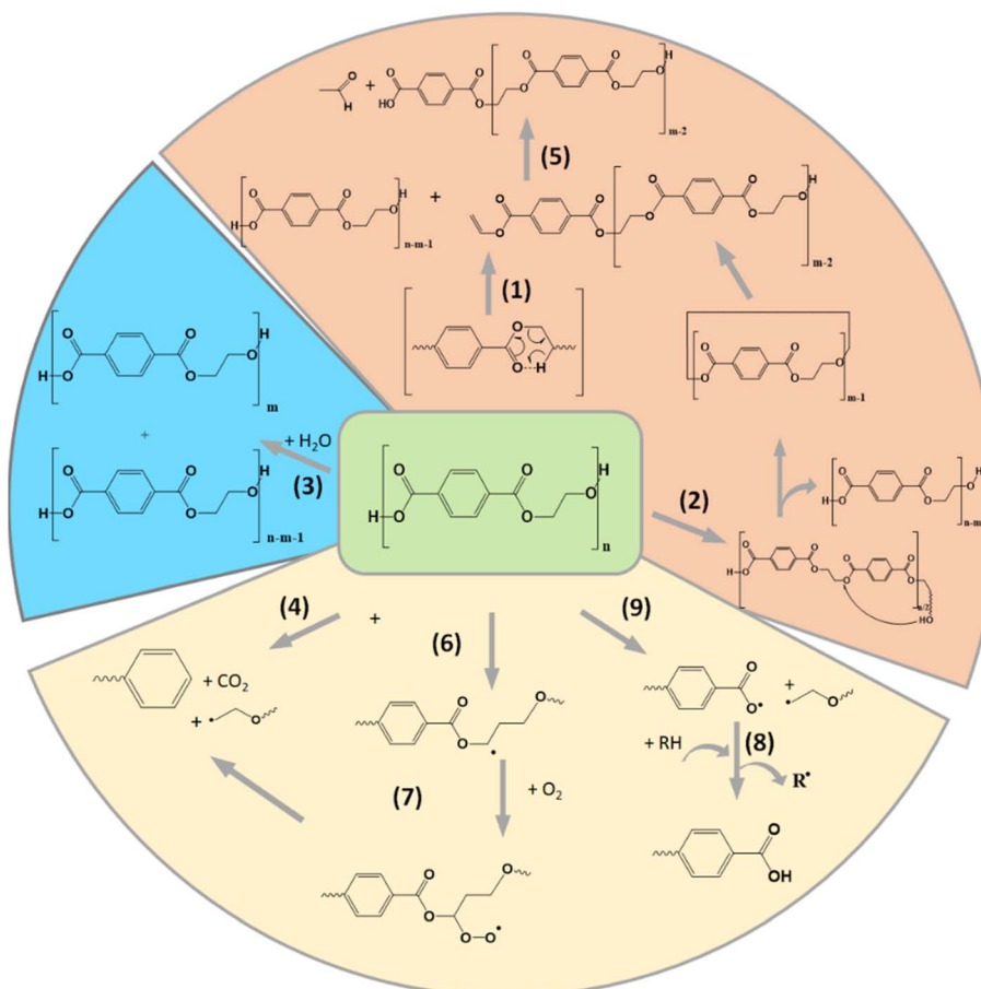
Fig. 2 Examples of PET (lumped) degradation reactions as likely encountered during mechanical recycling and end-of-life: (1) mid-chain driven ester rearrangement or net results of fission and βH-abstraction, defining radical-based ester rearrangement, e.g. thermal or thermomechanical; (2) alternative end-driven ester rearrangement with intermediate cyclization; (3) hydrolysis; (4) carboxylation with CO 2 formation; (5) volatile (aldehyde) formation; (6) hydrogen abstraction; (7) oxygen propagation as part of thermo-oxidative degradation; (8) chain transfer; (9) photo-oxidative scission.
