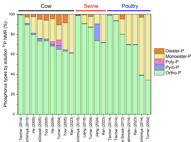
Fig. 3 Overview of phosphorus types in cow, swine, and poultry manures as analyzed by liquid phase 31 P NMR spectroscopy using data from various sources. 21,36,42,45,57,61,77,90–94
